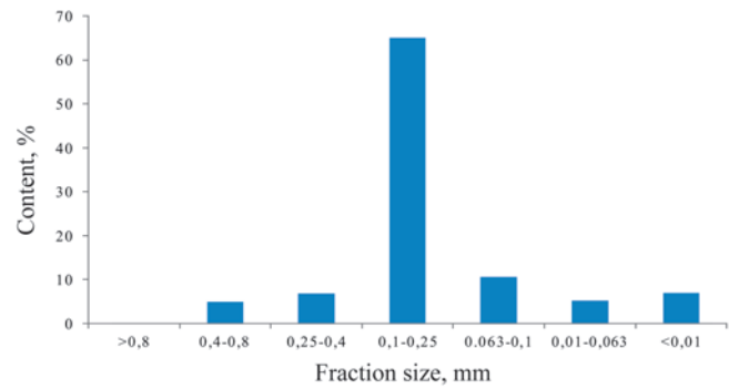
Fig. 5 The average histogram of the particle size distribution of the productive formation of well 15
