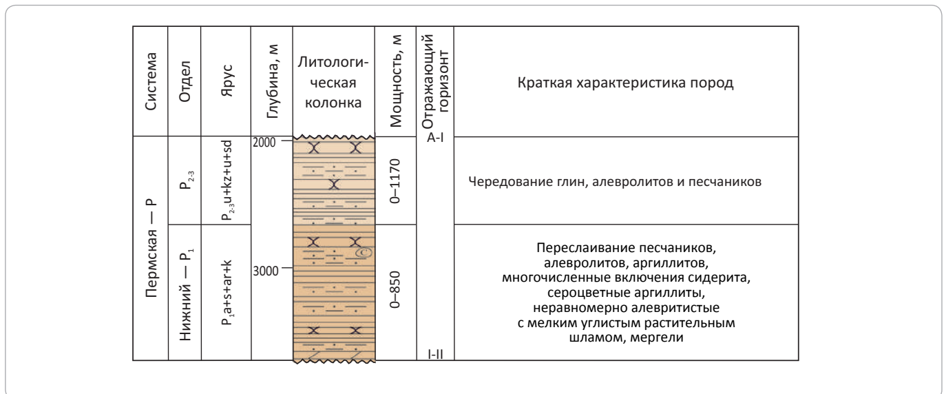
Fig. 4. Fragment of lithostratigraphic section across the western shoulder of the Korotaikhinsky depression (I.A. Marakova)
