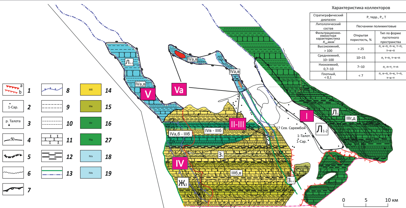
Fig. 8. Sketch map of lithofacies with P 2-3 kz+sd tectonic-facies and dynamic zones delineated (compiled by I.A. Marakova, using of archive materials from OOO Severgeofizika and OOO TP NIC)
