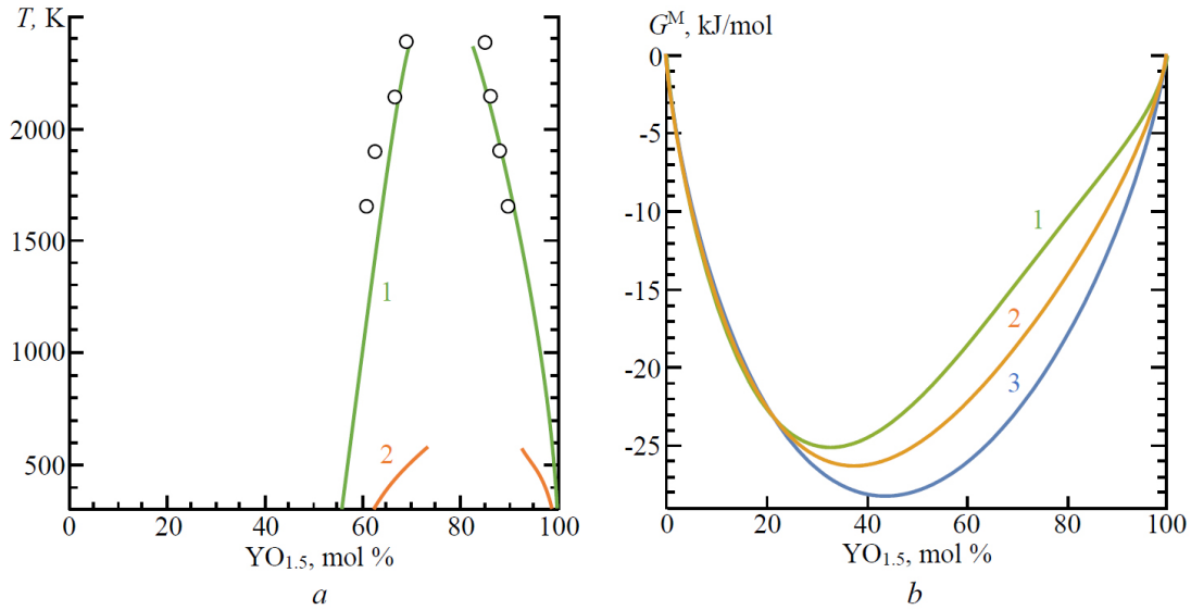
FIG. 2. a) Part of the ZrO_2 - YO_{1.5} calculated phase diagram. Points denote experimental data adopted from the paper [36]. Curve 1 was calculated at C^\nu = 1 , curve 2 was calculated at C^\nu = 0.6 (see equations (2) and (3)). b) The Gibbs energy of mixing G^M at 1 - C^\nu = 1 , 2 - C^\nu = 0.6 , 3 - C^\nu = 0.2
