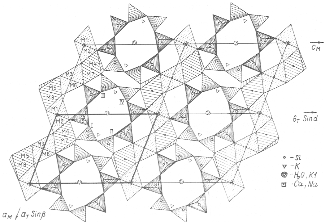
FIG. 3. Projection of the canasite structure along the elongated axis. Triclinic cell is shown by thick line. I, II, III, IV mark the four pectolite-like chains forming the \text{Si}_{12}\text{O}_{30} tube. M(1) , M(2) are alternately Na and Ca octahedra, while M(3) – M(8) are mixed Ca, Na positions.
