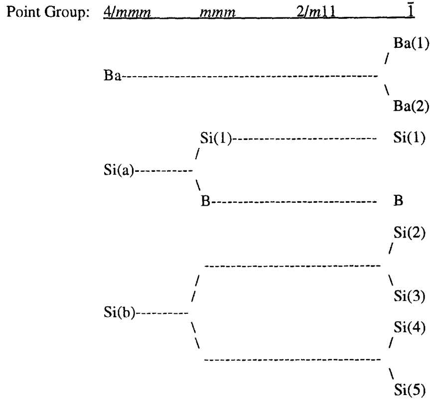
FIG. 2. Splitting of hyalotekite atom sites as the symmetry is lowered stepwise from I4/m\bar{m}m to \bar{1} . (a) cations, (b) (opposite) anions. Note: Pb site splits in a similar fashion to the Ba site. The Ca and F sites do not split.
