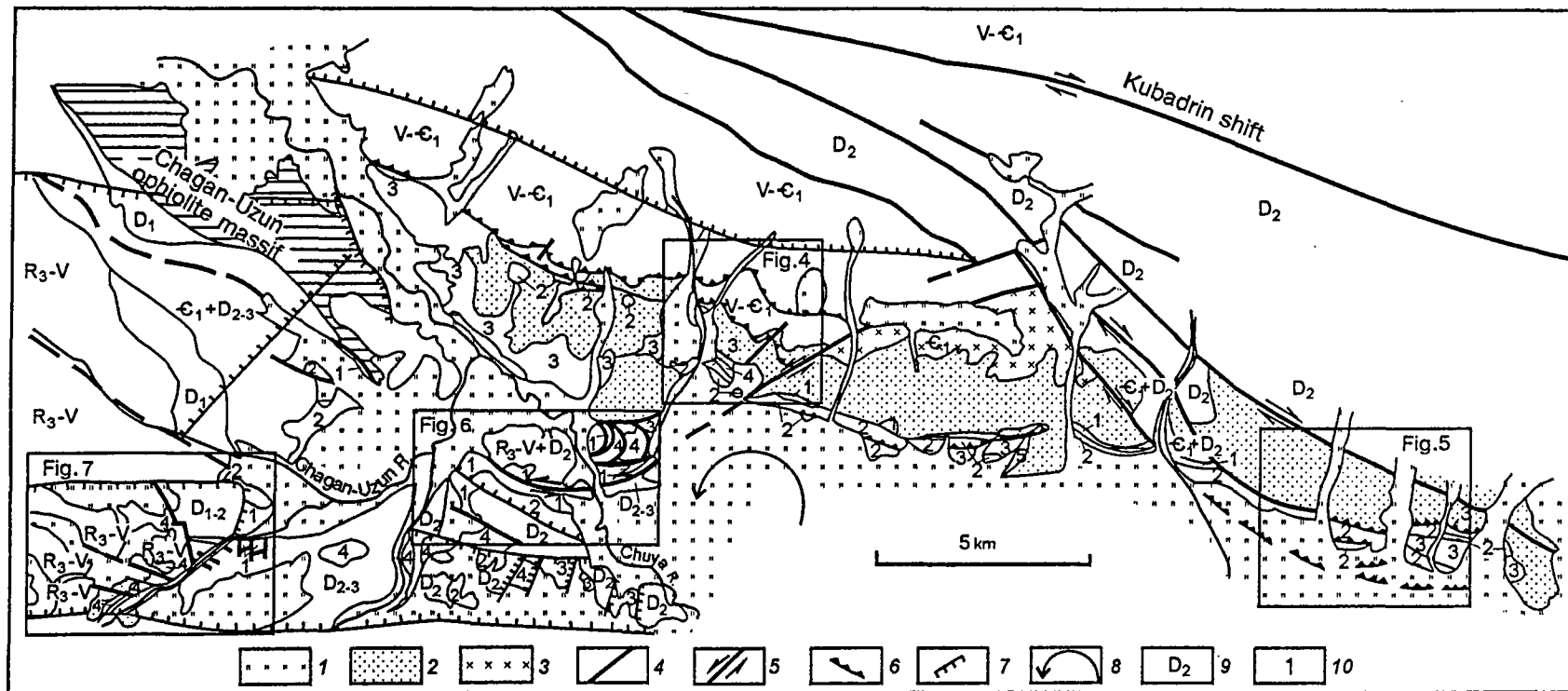
Fig. 3. Neotectonic framework of southeastern Gorny Altai. 1 – Quaternary deposits ( Q_{2-3} ), 2 – Terek-Bashkaus Formation ( N_2^2-Q_1 ), 3 – Tadzhlilin massif, 4 – faults (PZ), 5 – strike-slip faults ( Q_1 ), 6 – thrusts ( Q_1 ), 7 – reverse faults ( Q_1 ), 8 – rotation of southern Chuya depression in the latest Miocene – earliest Pliocene, from paleomagnetic data, 9 – pre-Cenozoic rocks, 10 – localization of sites. Numerals stand for: 1 – Karachum Formation ( P_3^2-3 ), 2 – Kosh-Agach Formation ( P_3N_1^{1-2} ), 3 – Tueryk Formation ( N_1^{1-3} ), 4 – Kyzyl-Gir Formation ( N_1^3 ), 5 – Beken Formation ( N_1^2 ).
