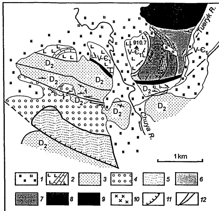
Fig. 6. Geological framework of the Krasnaya Gorka site (location see in Figs. 2 and 3). 1 – terrace deposits (Q 2-4 ), 2 – Vendian-Early Cambrian lavas and limestones (V-E 1 ), 3 – red-color rocks (D 2 ). Formations: 4 – Karachum (P 3 2-3 ), 5 – Kosh-Agach (N 1 1-2 ), 6 – Tueryk (N 1 1-3 ), 7 – Kyzyl-Gir (N 1 3 N 1 4 ), 8 – Bashkaus (N 2 2 -Q 1 ), 9 – serpentinite melange, 10 – stromatolites of the Kyzyl-Gir Formation, 11 – normal faults, 12 – strike-slip faults.
