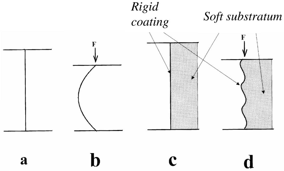
Fig. 6. Buckling instability for an anisodiametric body in a free state (a, b) and on a soft substratum (c, d).
