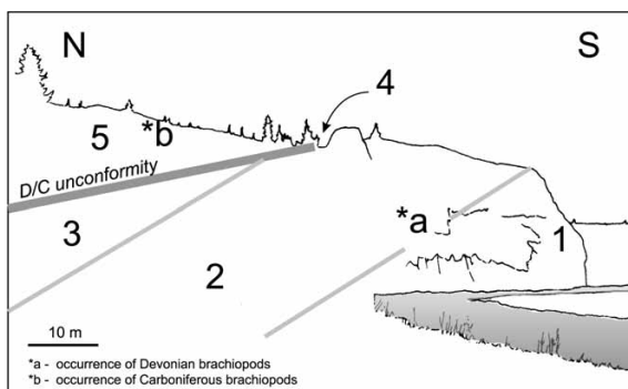
Fig. 3. Schematic location of the main lithological units at Locality 9 (morphology based on Pl. 1, Fig. 1)
