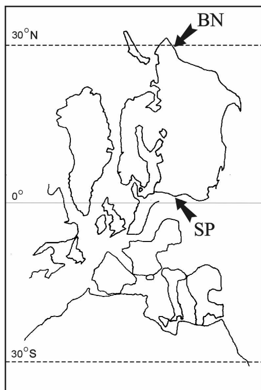
Fig. 1. Palaeogeographical position of Laurussia in the Late Viséan (after SCOTSE & MCKERROW 1990). Arrows indicate regions discussed in the paper: Bol'shaya Nadota section (BN) and Southern Poland (SP)
