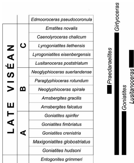
Fig. 9. Ammonoid zonation of the Rhenish Massif (Germany), after KORN (1996) with ranges of the genera which compose the Olyssa Hill fauna
