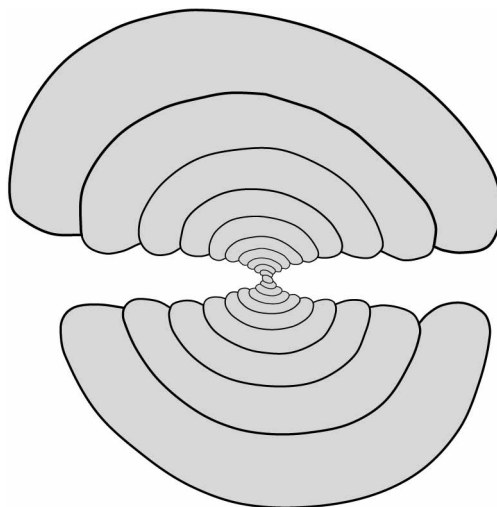
Fig. 7. Cross-section of Goniatites olysya sp. n.; paratype GPIT 1874-17; \times 2
