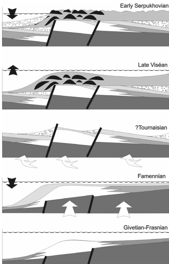
Fig. 6. Scheme of development of the Bol'shaya Nadota Carbonate Complex (description in text)
