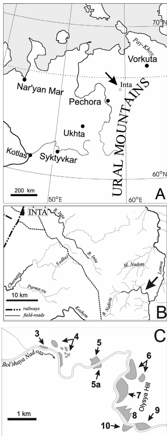
Fig. 2. Location of the Bol'shaya Nadota section (A, B) and outcrops described in text (C)
