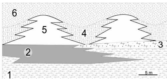
Fig. 4. Schematic relationships of the main lithological units at Locality 6 (description of units in text)
