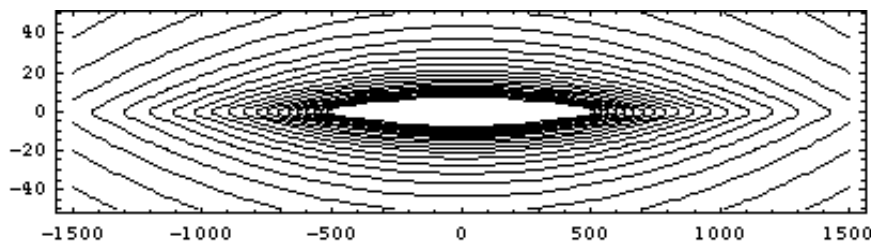
Figure 4. Vertical cross-section of isolines of the magnetization field structure function/variogramme in the crust (assuming the Curie depth \approx 100 km); horizontal and vertical scales are given in km, H_z = 2 , spheroscale = 40 000 km. Scale in km, aspect ratio is 1/4. This is based on eq. (16b) and shows the typical magnetization structures that dominate the second-order statistics.
