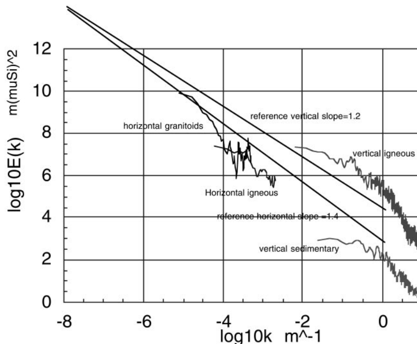
Figure 5. Power spectra of horizontal and vertical magnetic susceptibilities taken from Pilkington & Todoeschuk (1995) and Pilkington & Todoeschuk (1993), respectively [a typographic error in the measurement units in Pilkington & Todieschuck (1995) was corrected following a discussion with M. Pilkington]. The former have been multiplied by 2\pi k so as to yield angle-integrated rather than angle-averaged spectra. The straight lines show the reference slopes \beta_x = 1.2 (vertical), \beta_x = 1.4 (horizontal) with H_z = (1.4 - 1)/(1.2 - 1) = 2 and spheroscale at 10^5 km. Note that for the borehole data there is a large variation in spectral density depending on rock type, but that the vertical igneous and horizontal igneous do indeed show signs of intersecting at scales of 10^5 km or so, compatible with the indirect spheroscale estimates given by the stratified scaling model.
