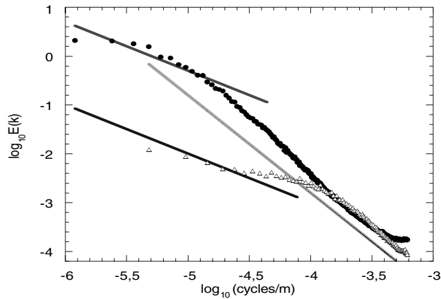
Figure 1. Power spectra of aeromagnetic anomaly fields from two regional surveys, shown as triangles and circles, data sets #1, #2, respectively. Superimposed for reference are line segments with the theoretical high- and low-wavenumber exponents, \beta_h=2 and \beta_i=1 (see Section 6). The spectra have been normalized so that the high-wavenumber regions roughly coincide.
