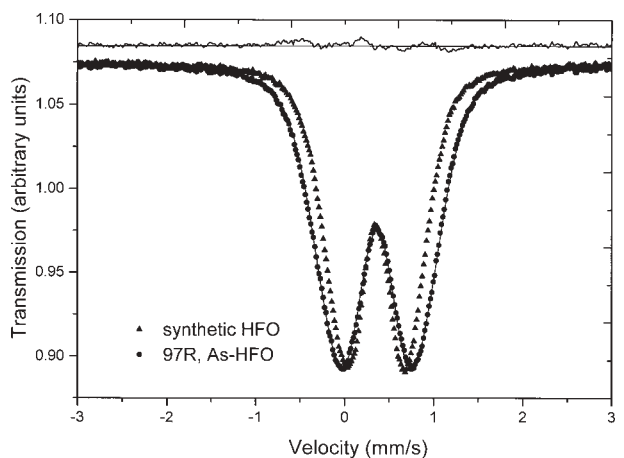
FIGURE 5. RT Mössbauer spectrum of As-HFO sample 97R, compared to that of a synthetic HFO sample ( [\text{Fe}] = 10^{-3} M , \text{pH} = 9 ). The fit to the 97R spectrum, that is described in Tables 3 and 4, is shown by a solid line running through the data points and the corresponding residual is shown above the spectra, using the same vertical scale. The two spectra have been rescaled and shifted to facilitate comparison.
