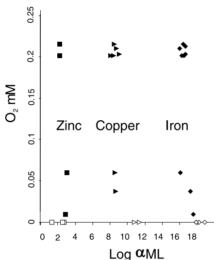
Fig. 10. Relative stability of natural complexes in the water column and the fluffy layer, expressed as \log \alpha_{ML} . The results of all three profiles at the Blinkerhügel site are shown (squares = zinc; triangles = copper; rhombs = iron; open symbols represent the fluffy layer).
