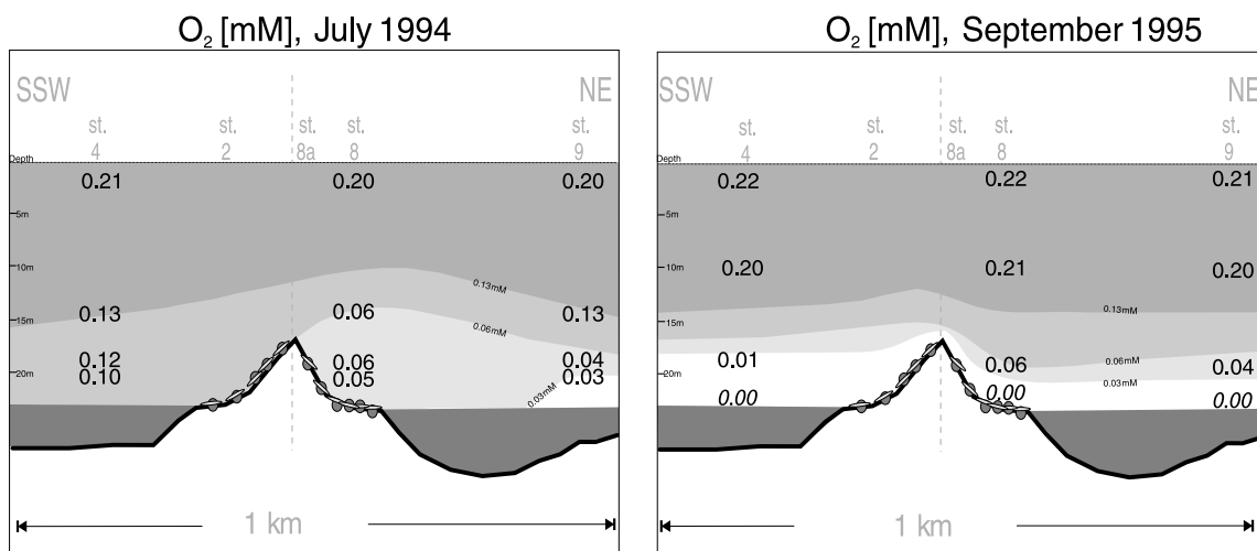
Fig. 3. Oxygen concentration (mM) at the Blinkerhügel area in July 1994 and September 1995 (italic: fluffy layer).
