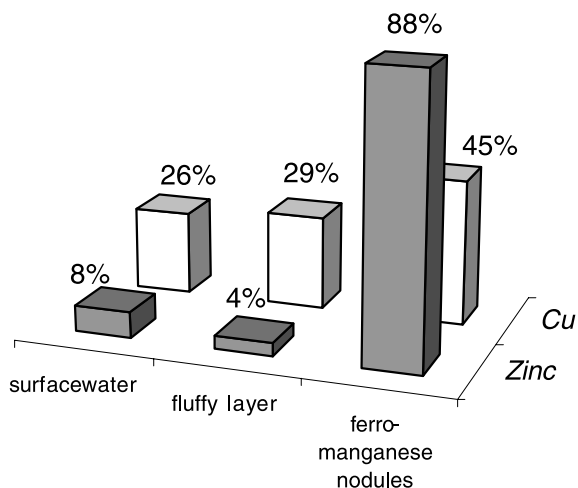
Fig. 11. Relative distribution of zinc and copper in the surface water, the fluffy layer and the ferro-manganese nodules.
