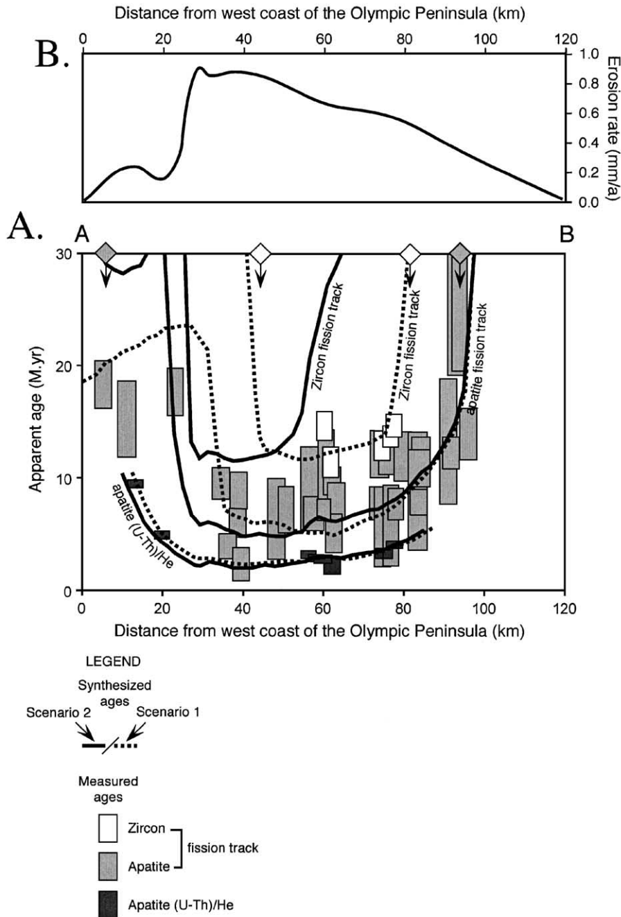
Fig. 3. (A) Thermochronological age variation across the Olympic orogen plotted as apparent age vs. distance along section A–B in Fig. 2. Zircon fission track ages came from Brandon and Vance (1992) and Garver and Brandon (1994), apatite fission track ages from Brandon et al. (1998) and Roden-Tice (unpublished data), and (U–Th)/He ages are taken from Batt et al. (2001) and unpublished data of the authors. The shaded symbols straddling the upper margin of the chart indicate the transition to inherited or ‘unreset’ ages off the scale of this figure for the respective fission track data sets. The curves plotted represent the results of 2-D dynamical models discussed in detail by Batt et al. (2001), comparing the relative thermochronological implications of kinematic scenarios 1 and 2 (Fig. 2), as discussed in the text. (B) Recent erosion rates across the Olympic Peninsula, calculated from the apatite fission track ages and deformed and offset river terraces, after Pazzaglia and Brandon (in review).
