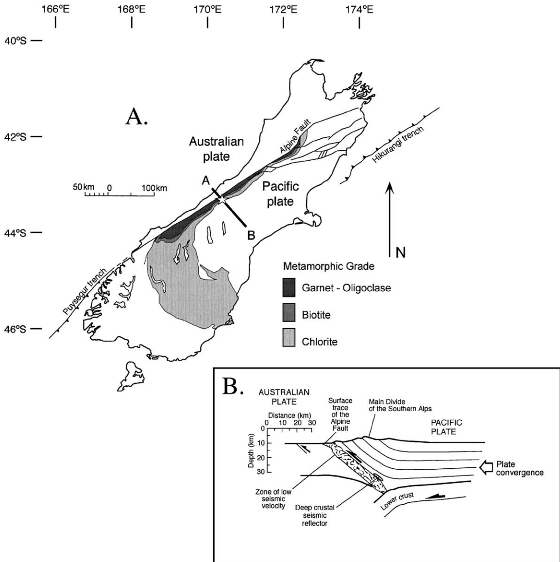
Fig. 5. (A) Major geological features of the Southern Alps and localities mentioned in the text, simplified from Grapes and Watanabe (1992). The star shown in the central region of the orogen indicates the approximate location of the samples discussed in relation to Fig. 6. Line A–B indicates the approximate location of the section shown in panel B. (B) Figurative section summarizing the geophysical constraint of the crustal structure beneath the Southern Alps. This illustrative section is a composite sketch, drawing on the results of Reyners and Cowan (1993), Smith et al. (1995), Stern (1995), and Davey et al. (1995).
