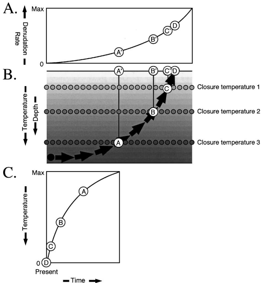
Fig. 1. Thermochronological significance of the material convergence relative to the denudational and thermal framework of a deforming region. Note that although figurative, the processes and effects illustrated are derived from published (Batt and Braun, 1997, 1999; Batt et al., 2001) and unpublished numerical modeling works of the authors. (A) Assumed variation in erosion rate across the area of interest, (B) regional thermal structure and the material path taken by a selected sample during its passage through the deforming region. Arbitrary closure temperatures are shown for three ‘thermochronometers’, as discussed in the text. (C) Variation in the temperature experienced over time by the particle illustrated in panel B. Note the progressive acceleration in the cooling rate. This is caused by spatial rather than temporal variation in the exhumation rate (panel A), and thus, illustrates the caution required in attaching the dynamic significance to such features.
