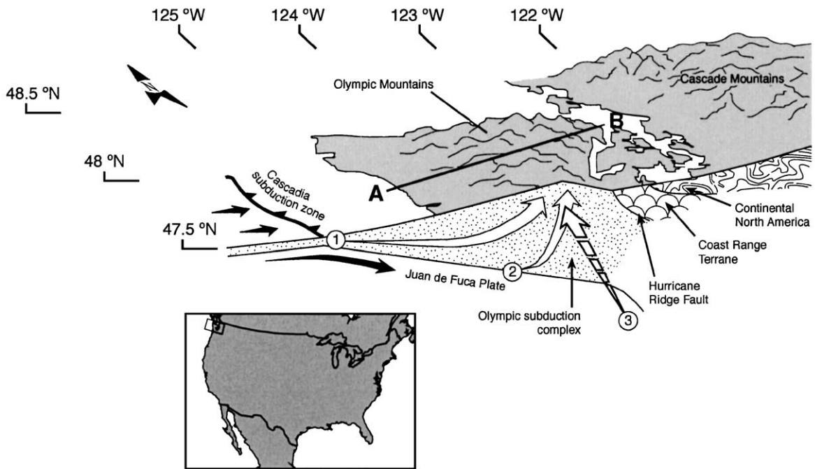
Fig. 2. Key geographical features of the Cascadia margin of North America, incorporating a figurative cross-section illustrating the structural and tectonic nature of the Olympic section of the Cascadia wedge, after Brandon et al. (1998). Line A–B indicates the approximate position of the thermochronological transect shown in Fig. 3. The white arrows illustrate the material flux paths suggested by the competing hypotheses of the Olympic orogen kinematics: (1) frontal accretion of the incoming sedimentary section of the Juan de Fuca plate at the toe of the Cascadia wedge (e.g. Davis and Hyndman, 1989), (2) underplating of subducted material at depth beneath the orogen (e.g. Clowes et al., 1987; Brandon and Calderwood, 1990), and (3) margin-parallel transport (e.g. Beck, 1991; McCaffrey and Goldfinger, 1995; McCaffrey, 1996; McCrory, 1996; Wang, 1996). Note that arrows 1 and 2 are in, and arrow 3 is perpendicular to, the plane of the illustrated section.
