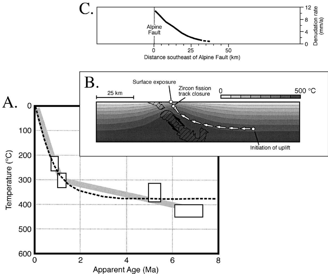
Fig. 6. Interpretation of cooling histories experienced in the Southern Alps. (A) Grey curve shows the cooling history experienced by rocks adjacent to the Alpine Fault in the central Southern Alps (Fig. 5), after Tippett and Kamp (1993). Constraints indicated by the white boxes correspond to, in order of increasing temperature, zircon fission track ages (Tippett and Kamp, 1993), biotite and muscovite K–Ar ages (Adams, 1981), and the inferred pre-uplift temperature of the region (Tippett and Kamp, 1993). The overlain black dotted curve indicates the cooling history of a particle passing through a 2-D simulation of the Southern Alps over 5 Ma, as indicated in panel B. (B) Numerical model results illustrating the exhumation history of a particle passing through a convergent orogen modeled on the Southern Alps, after Batt (1997) and Batt and Braun (1997, 1999). Convergence is at 10 mm/year, horizontal and vertical scales are equal, and the thermal structure shown is that developed after 5 Ma of deformation. The crosshatched region marks the peak strain rates in the model after 5 Ma and is interpreted to equate with the Alpine Fault for the Southern Alps (Fig. 5B). The white arrows show the exhumation trajectory of a selected particle. Also shown are the location at which the indicated particle begins to be exhumed and the site at which it undergoes closure for the zircon fission track chronometer, as discussed in the text. (C) Exhumation rates across the central Southern Alps as calculated from the zircon fission track ages by Tippett and Kamp (1993). Rates are plotted relative to the Alpine Fault, with the same horizontal scale as in panel B, to allow direct comparison between the two panels.
