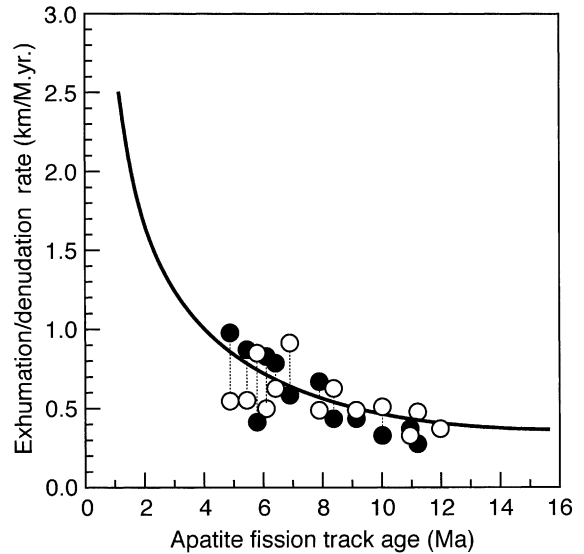
Fig. 4. Relationship of modeled fluorapatite fission track ages at the surface of the Olympics to exhumation rate. Solid line marks the 1-D relationship, calculated after Brandon et al. (1998), for a 20-km-thick crustal layer, assuming the thermal diffusivity of 20 \text{ km}^2/\text{Ma} and a thermal structure at equilibrium, as discussed in the text. Paired circular symbols represent the corresponding relationship for individual samples analyzed in a 2-D model of the Cascadia accretionary wedge-forearc system (Batt et al., 2001) (Fig. 3). Open circles mark the denudation rate at the site of a sample's exposure at the surface, with filled circles marking the exhumation rate experienced at the modeled time of closure.
