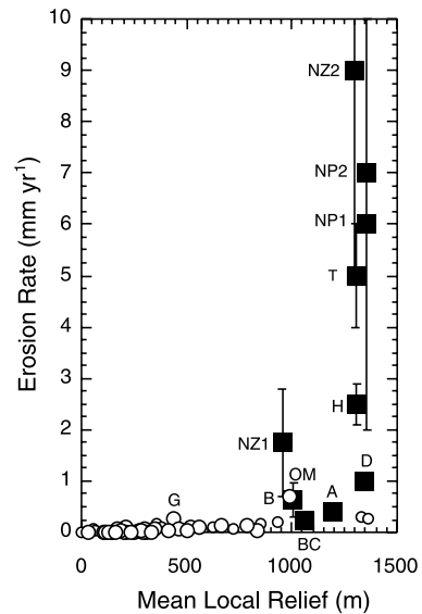
Fig. 3. Same data as in Fig. 2 but with the addition of solid squares representing mean values of long-term erosion rates (error bars span range of data) reported in published sources for the tectonically active convergent areas of the southern island of New Zealand Alps (NZ1 from Tippett and Kamp [53]), the western slope of the New Zealand Alps (NZ2 from Hovius et al. [48]), central Himalaya (H) [52], the Himalayan portion of the Indus River drainage basin from (NP1 from Burbank et al. [12] and NP2 from Shroder and Bishop [49]), the Olympic Mountains (OM) [39], Taiwan (T) [46], the Denali portion of the Alaska Range (D) [47]; and the European Alps (A) [50]. Data points from Fig. 3 for the Ganges (G) and Bramaputra (B) rivers are shown for reference. The extent of the area of active tectonic uplift for Central Himalaya, Olympic Mountains, and Taiwan was defined by areas above 200 m elevation. The areas analyzed for the New Zealand and European Alps were based on the area of dissected uplands that physiographically define each range.
