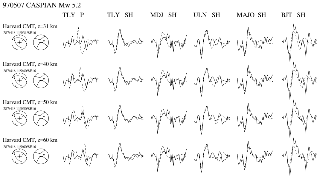
Figure A11. Waveforms for an earthquake of M_w 5.2 on 7 May 1997 on the Apsheron–Balkhan sill (Fig. 6). There were insufficient clear seismograms for a full inversion, but the depth of 50 \pm 5 km can be confirmed. The four lines of waveforms show synthetics calculated at 31, 40, 50 and 60 km using the Harvard CMT orientation and M_0 with a short (2 s) impulsive time function. The interface between the top layer ( V_p 6.5 km s -1 and the half-space of V_p 8.1 km s -1 was at 30 km and a water depth of 500 m was included. Particularly clear surface reflections are seen at TLY (P) and BJT (SH). The Harvard depth was 63 km (58 per cent double-couple).
