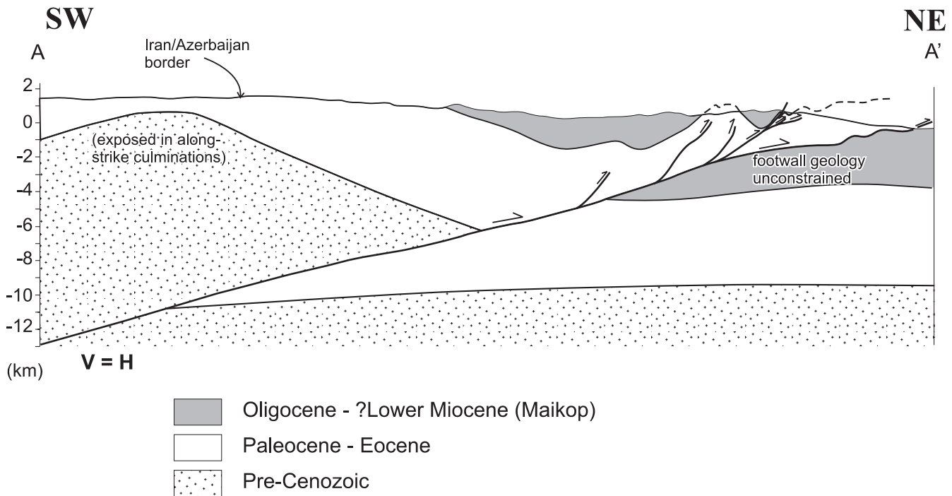
Figure 10. A schematic geological cross-section of the NE Talesh in Azerbaijan (see Fig. 3 for location), drawn to reconcile the earthquake and surface data. Most large earthquakes are on the basement thrusts at 10–20 km depth beneath the Iran–Azerbaijan border, whereas the surface folding in the young sediments occurs further NE and offshore, where the thrusts reach shallower levels. The vertical and horizontal scales are equal.
