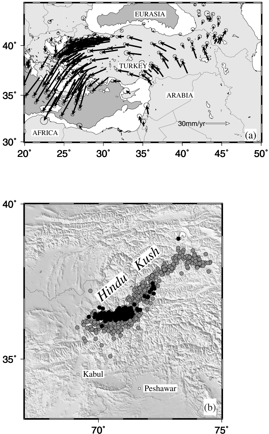
Figure 12. (a) GPS velocities in the eastern Mediterranean region relative to stable Eurasia, from McClusky et al. (2000). Bathymetry deeper than 2000 m is in grey. Note how the continued anticlockwise rotation of Turkey and SW motion of Greece will eventually isolate the eastern Mediterranean basin and surround it by continental material. (b) Earthquake epicentres in the depth range 100–200 km (grey) and deeper than 200 km (black) in the Hindu Kush. Data are from the catalogue of Engdahl et al. (1998) in the period 1964–1998. Note that in the west the slab defined by the earthquakes dips N, but in the east it dips SE (see also Pegler & Das 1998).
