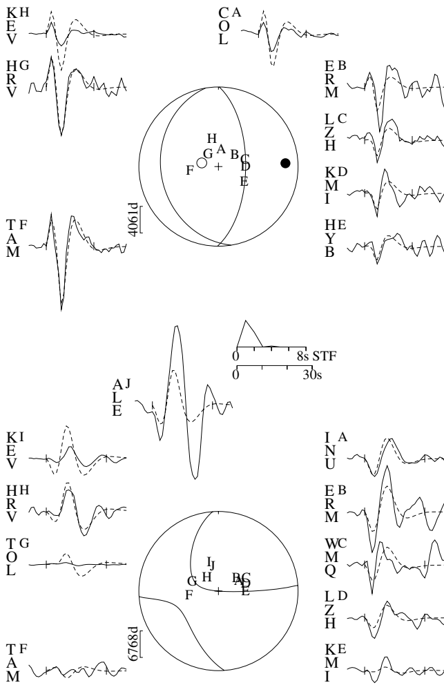
Figure A2. Minimum misfit solution for the earthquake of 1990 June 21 ( M_w 5.6), an aftershock of the 1990 June 20 Rudbar–Tarom earthquake ( M_w 7.3). This event shows N–S reverse faulting at the end of an E–W left-lateral strike-slip fault (Fig. 7a). Our solution is similar to that of Gao & Wallace (1995), who obtained 023/64/92/8 km/ 4.0 \times 10^{17} N m using a combination of regional and teleseismic waveforms, and similar in orientation to the Harvard CMT best-double-couple solution (351/68/76/15 km (fixed)/ 4.95 \times 10^{17} N m/53 per cent double-couple).
