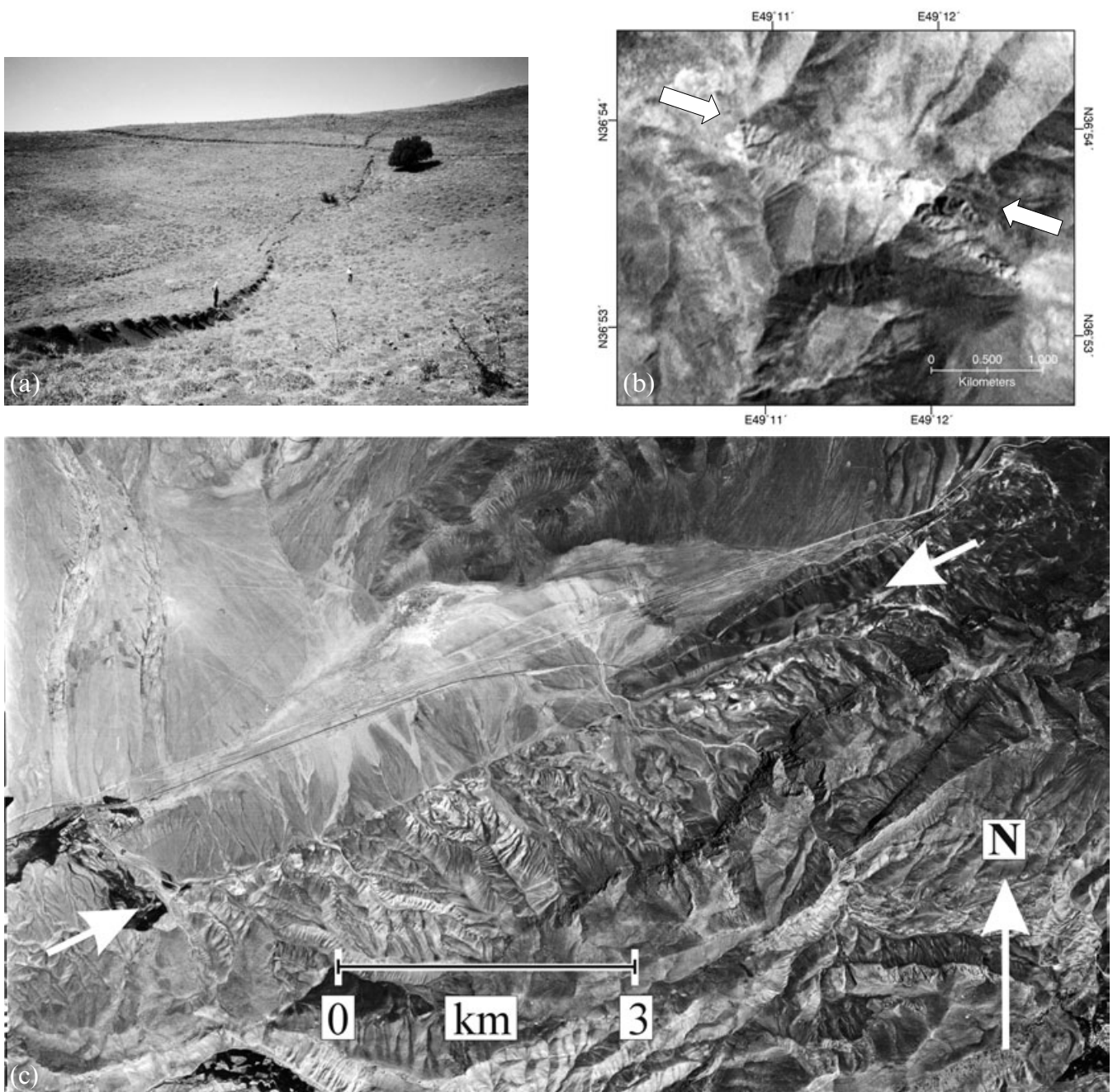
Figure 9. (a) The left-lateral surface rupture of the 1990 Rudbar–Tarom earthquake ( M_w 7.3) near Jaishabad ( 36^{\circ}54.0'N , 49^{\circ}10.1'E ) in the western Alborz, photographed in 2000 September, 10 years after the earthquake. This rupture connects the Kabateh and Baklor fault segments described by Berberian et al. (1992), which are now known to be continuous. The view is to the west, with the north side dropped by \sim 1 m, in the opposite sense to the local topography (see Fig. 9b). The left-lateral component was visible on the ground, but could not be measured accurately 10 years after the earthquake. (b) LANDSAT 7 TM image of the 1990 Rudbar–Tarom strike-slip fault at Jaishabad (Fig. 9a). The fault is visible between the white arrows, mostly because its vertical component (down to the north) is in the opposite sense to the local topography, and has caused streams crossing the fault from N to S to incise on the southern side. This is one of the very few locations where the 1990 ruptures are clearly associated with a feature that is clear in the geomorphology. (c) Aerial photo of the left-lateral Firuzkuh fault, near 53^{\circ}E (see Fig. 7b and Berberian et al. 1996). The fault is visible between the white arrows. (d) Air photo of the left-lateral Astaneh fault near 53.5^{\circ}E (Fig. 7b). The Astaneh fault runs between the big white arrows. Smaller arrows show beheaded streams flowing from NW to SE, now offset in a left-lateral sense.
