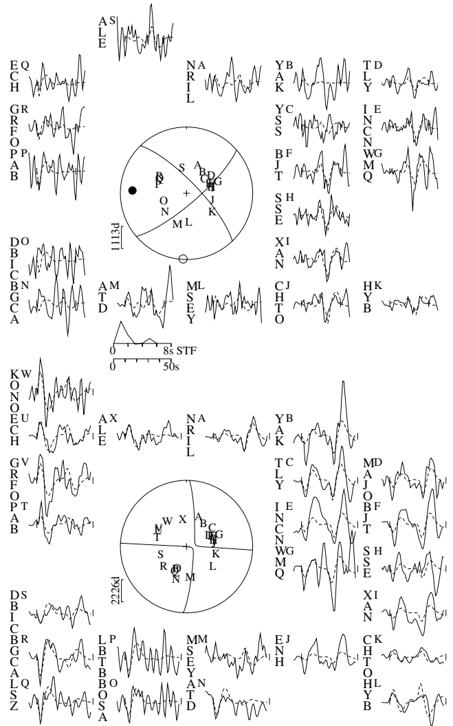
Figure A7. Minimum misfit solution for a deep (~61 km) strike-slip event near the Apsheron-Balkhan sill (Fig. 6). The earthquake was only M w 5.3 and some waveforms are noisy, as well as quite small in amplitude near nodal planes. Nonetheless, the clear surface reflections in the P waves at eastern stations (e.g. SSE, XAN, CHTO) and in the SH waves in the NE and SE quadrants (e.g. YAK, TLY, XAN, HYB) constrain the depth to within ~±5 km. Synthetics were calculated with the interface between the top layer (V p 6.5 km s -1 ) and half-space (V p 8.1 km s -1 ) at 30 km, and with a water depth of 500 m. Our solution is similar to that of the Harvard best-double-couple (314/75/-42/26 km/2.15 × 10 17 N m/57 per cent double-couple) except for the centroid depth, which trades off against moment.
