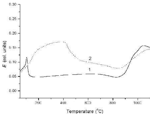
Figure 7. Emanation thermal analysis data of (\text{NH}_4)_2\text{SiF}_6 -treated vermiculites. Curve 1: \text{Na}^+ -vermiculite treated with (\text{NH}_4)_2\text{SiF}_6 and totally saturated with \text{Na}^+ ions ( \text{Na}^+\text{-V}_{\text{dealum}} ). Curve 2: \text{Na}^+ -vermiculite treated with (\text{NH}_4)_2\text{SiF}_6 and partially saturated with \text{Na}^+ ions ( \text{NH}_4^+/\text{Na}^+\text{-V}_{\text{dealum}} ).
