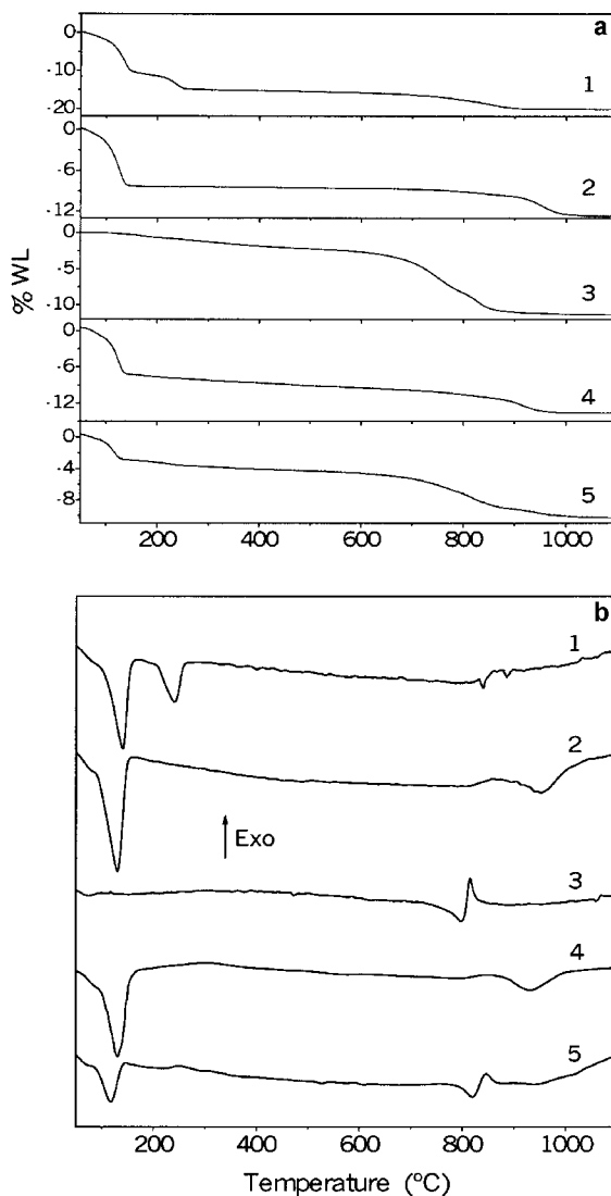
Figure 2. Thermogravimetry (a) and DTA (b) results of vermiculite samples measured during heating in air. (a) TG curves of Mg^{2+} -vermiculite (curve 1), Na^+ -vermiculite (curve 2), NH_4^+ -vermiculite (curve 3), Na^+ -vermiculite treated with (NH_4)_2SiF_6 totally re-saturated with Na^+ ( Na^+ -V dealum , curve 4), and Na^+ -vermiculite treated with (NH_4)_2SiF_6 partially re-saturated with Na^+ ( NH_4^+/Na^+ -V dealum , curve 5). (b) DTA curves of Mg^{2+} -vermiculite (curve 1), Na^+ -vermiculite (curve 2), NH_4^+ -vermiculite (curve 3), Na^+ -vermiculite treated with (NH_4)_2SiF_6 totally re-saturated with Na^+ ( Na^+ -V dealum , curve 4), and Na^+ -vermiculite treated with (NH_4)_2SiF_6 partially re-saturated with Na^+ ( NH_4^+/Na^+ -V dealum , curve 5).
