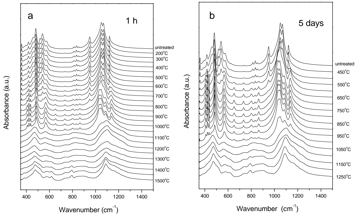
Figure 2. Infrared spectra (KBr pellets) in the region 350\text{--}1500\text{ cm}^{-1} of pyrophyllite EM08 samples (40–60 mesh) annealed in temperature range: (a) 200\text{--}1500^\circ\text{C} for 1 h; (b) 450\text{--}1250^\circ\text{C} for 5 d.
