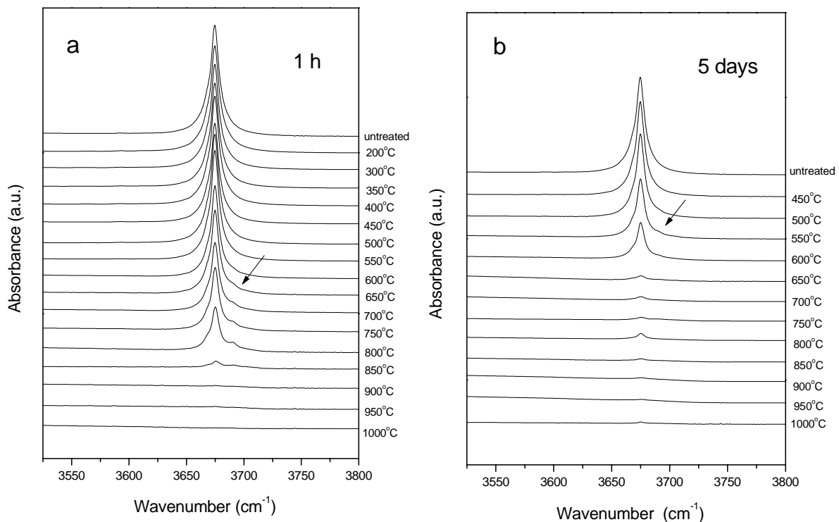
Figure 3. Infrared spectra (KBr pellets) in the region 3525\text{--}3800\text{ cm}^{-1} of pyrophyllite EM08 samples (40–60 mesh) annealed in temperature range: (a) 200\text{--}1000^\circ\text{C} for 1 h; (b) 450\text{--}1000^\circ\text{C} for 5 d. The arrows indicate the extra peak at 3690\text{ cm}^{-1} .
