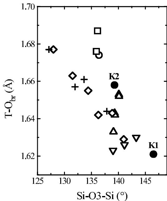
Fig. 3. Values of T-O_{br} plotted against the Si-O3-Si angle. The filled circles refer to the synthetic clinopyroxene crystals of this study. Empty symbols refer to published data (Cameron & Papike, 1981). Circles, natural K-rich diopside (Harlow, 1996); squares, C2/c pyroxenes with general formula CaM^{2+}Si_2O_6 ; up triangles, C2/c pyroxenes with general formula NaM^{3+}Si_2O_6 ; down triangles, C2/c pyroxenes with general formula LiM^{3+}Si_2O_6 ; diamonds, Pbc pyroxenes; crosses, P2_1/c pyroxenes.
