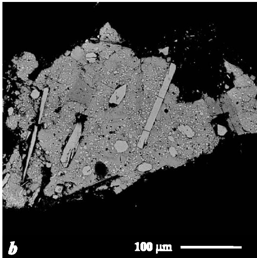
Fig. 1. BSE images of idiomorphic clinopyroxene crystals, coexisting with garnet (small idiomorphic equant grains in the matrix), produced in the runs (a) 688 (1310 °C, 60 mol. % \text{KAlSi}_2\text{O}_6 ) and (b) 650 (1350 °C, 70 mol. % \text{KAlSi}_2\text{O}_6 ). CamScan electronic microscope.
