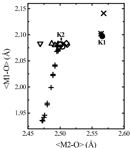
Fig. 2. Values of \langle M1-O \rangle distances in C2/c clinopyroxenes plotted against \langle M2-O \rangle distances. The filled circle refers to the synthetic clinopyroxene crystals of this study. Open symbols are literature data, as follows: circle, natural K-rich diopside (Harlow, 1996); square, diopside (Cameron et al. , 1973); down triangle, Di 66 En 34 (Tribaudino et al. , 1989); up triangles, Di 100 , Di 90 En 10 , Di 80 En 2 (Bruno et al. , 1982); diamonds, (Ca,Sr)-clinopyroxenes (Benna et al. , 1987); crosses (+) natural clinopyroxenes of the augite-jadeite join (Boffa Ballaran et al. , 1998); star, NaScSi 2 O 6 (Hawthorne & Grundy, 1973); cross (x), NaInSi 2 O 6 (Hawthorne & Grundy, 1974).
