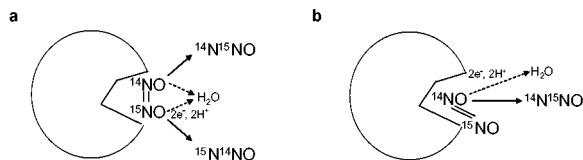
Figure 6 Simultaneous (a) versus sequential (b) binding of NO to NOR. Formation of predominant N_2O isotopologue(s) indicated for each mechanism: Simultaneous binding leads to equivalent fractionation at N^\alpha and N^\beta ; sequential binding leads to greater fractionation at N^\beta .
