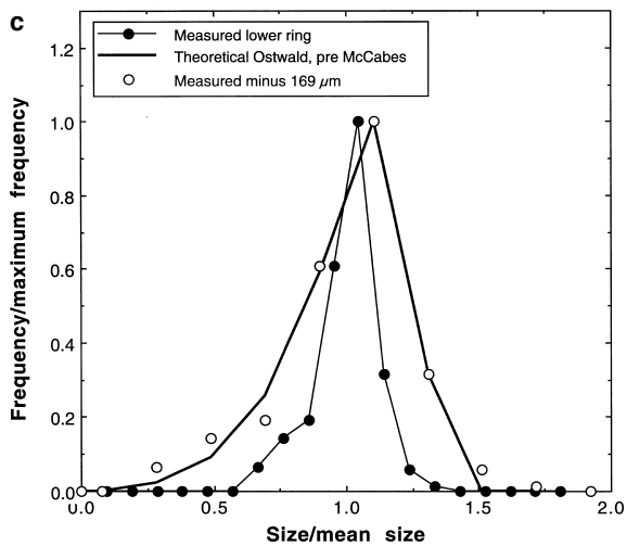
FIGURE 4. CSD measured for calcite grown in a 30 mm straight column: (a) upper Liesegang ring; (b) middle Liesegang ring; (c) lower Liesegang ring plotted using reduced axes.
