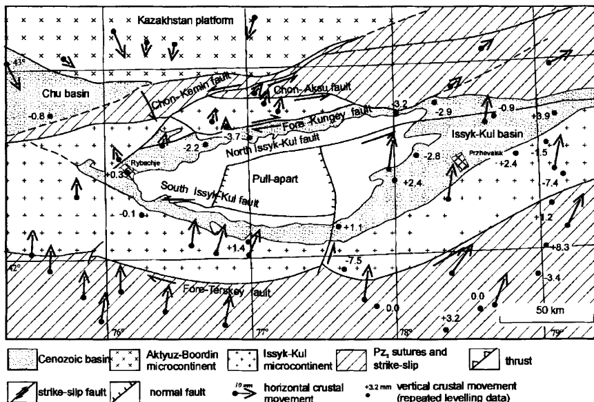
Fig. 8. Active strike-slip movements in northern Tien Shan (after geodetic surveys).
