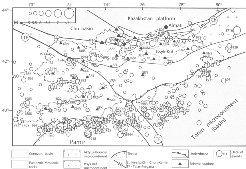
Fig. 6. Seismicity and tectonics of northern Tien Shan and neighbouring territories.
