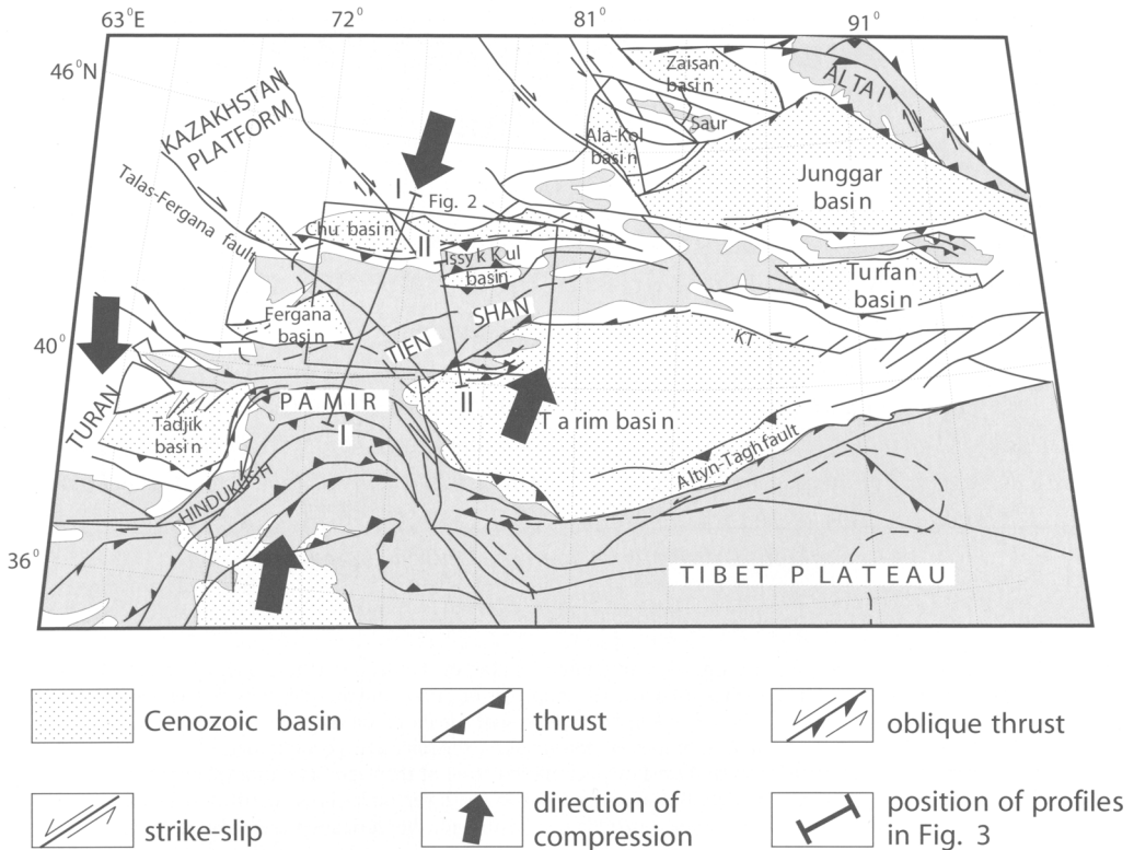
Fig. 1. Generalized tectonics of Central Asia (Tarim, Turfan, and Junggar basins and surrounding mountains). Modified after Cobbold and Davy (1988).
