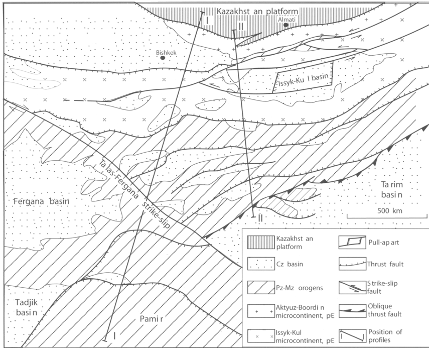
Fig. 2. Generalized tectonics of Tien Shan.
