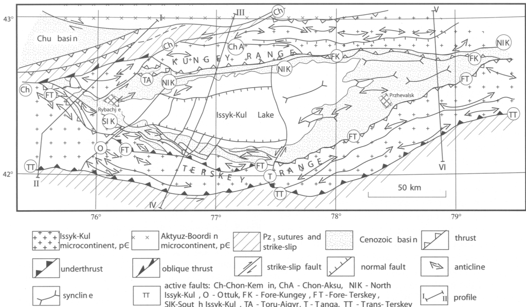
Fig. 4. Active tectonics of the northern Tien Shan around the Issyk-Kul basin.
