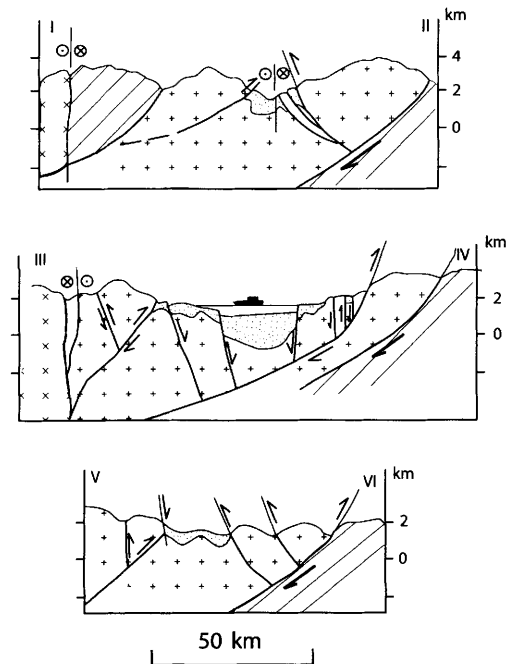
Fig. 5. Geological cross sections of different segments of northern Tien Shan around Issyk-Kul basin (for location of profiles see Fig. 4). Profile I–II (western Issyk-Kul microcontinent): Cenozoic sediments overthrust by basement rocks in a ramp structure. Profile III–IV (central Issyk-Kul microcontinent and Lake Issyk-Kul): reverse faulting at southern extremity of microcontinent. Profile V–VI (eastern Issyk-Kul microcontinent): basin fill is more strongly deformed in a half-ramp structure.
