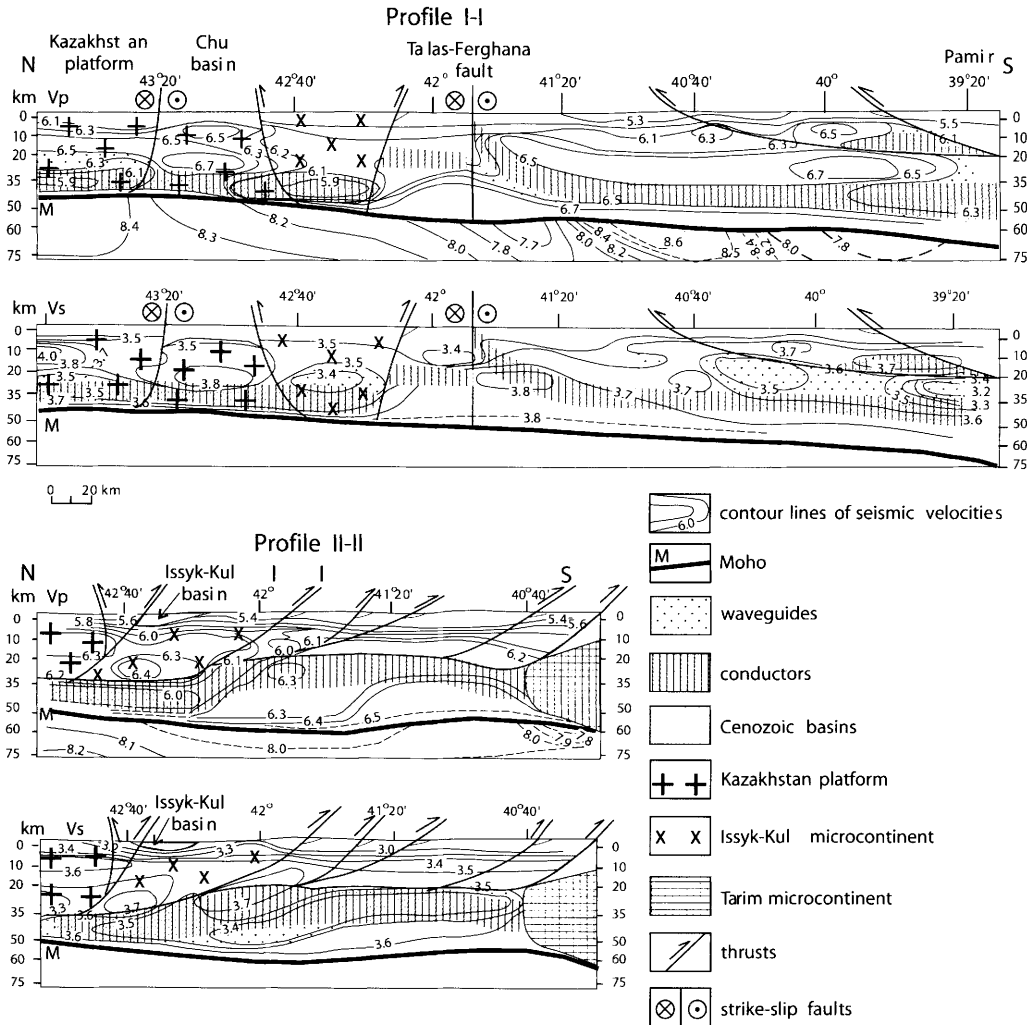
Fig. 3. Cross section of crust and upper mantle beneath Tien Shan, from P (Vp) and S (Vs) seismic velocities, along profiles Aktuz-Torugart (I) and Kindiktas-Karakul (II) (see Figs 1 & 2 for location). Modified after Bakirov et al. (1996).
