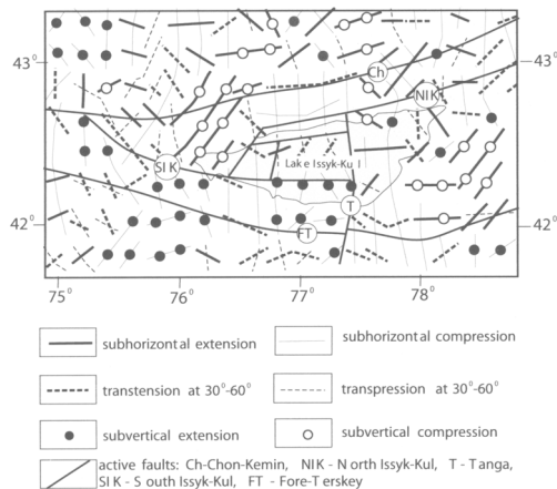
Fig. 7. Principal stresses in northern Tien Shan, from tensor analysis (see text for explanation).
