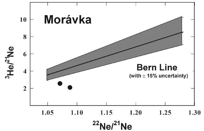
Fig. 2. Cosmogenic ^3\text{He}/^{21}\text{Ne} versus ^{22}\text{Ne}/^{21}\text{Ne} ratio in 2 Morávka meteorites and the empirical Bern line for chondrites without ^3\text{He} deficit.
