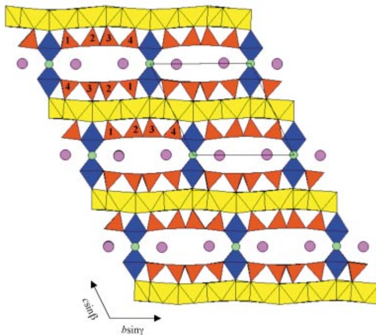
FIG. 3a. Crystal structure of triclinic astrophyllite-group mineral ( \bar{1} ) projected down [100] (unit cell outlined). O sheet: yellow, D : blue, T : red, A : magenta, B : green. The four T sites are indicated to show symmetry across the interlayer.
