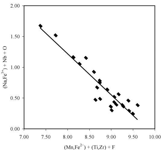
FIG. 16. Mechanism of substitution for the incorporation of Nb 5+ into the structure: M 2+ + M 4+ + F ⇌ (Na, Fe 3+ ) + Nb 5+ + O 2- (linear regression, R 2 = 0.870).
