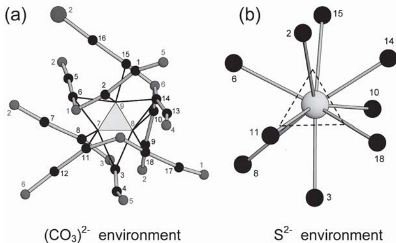
FIG. 5. The environments of the (\text{CO}_3) group (a) and the \text{S}^{2-} anion (b) in vasilyevite. Legend as in Figures 1, 3. Thin black lines: weak bonds from Hg atoms to O atoms of the (\text{CO}_3) group, yellow circle: \text{S}^{2-} atom, dashed triangle: outline of unoccupied (\text{CO}_3) triangle.
