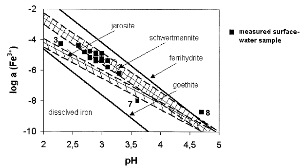
Fig. 2. Plot of the logarithm of the Fe 3+ activity (mean values of measured data) versus pH for surface waters of 17 AML (Niemegk is not presented, because no iron was detected). Solubility lines were calculated (using the Eqns. 1 to 4 in Table 2) for goethite (log a(Fe 3+ ) = 1.4–3pH), ferrihydrite (log a(Fe 3+ ) = 4.83–3pH), K-jarosite (mid-line: log a(Fe 3+ ) = -0.19–2 pH) and schwertmannite (mid-line: log a(Fe 3+ ) = 2.7–2.63 pH). Maxima and minima (dashed lines) for the solubility window of schwertmannite are the range log a(SO 4 2- ) = -1 to -1.5, that of jarosite -1.85 to -2.5 and for log a(K + ) = -3.5 to -4.07. Presented numbers correspond to lakes (Table 1), situated outside the stability window of schwertmannite.
