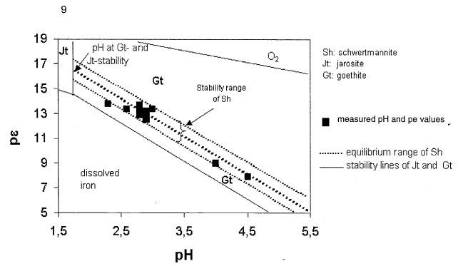
Fig. 9. pE-pH-diagram for the system K-Fe-SO 4 . Equilibration lines were calculated using the Eqns. 8 (schwertmannite), 10 (jarosite), and 11 (goethite). the stability line between Jt and Gt was calculated using KFe_3(SO_4)_2(OH)_6 \leftrightarrow 3 FeOOH + 3 H^+ + K^+ + 2 SO_4^{2-} ( \log K = -13.4 ) and between H 2 O and O 2 using 2 H_2O \leftrightarrow O_2 + 4 H^+ + 4 e^- ( \log K = 86.08 ). Datapoints represent measured values of pE and pH in the AML.
