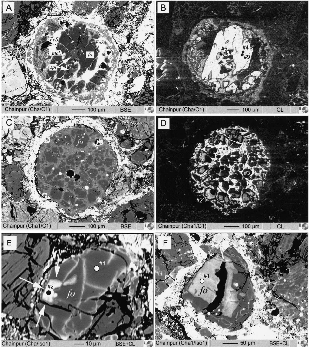
Fig. 2. Refractory forsterite grains from Chainpur (LL3.4). Numbers refer to ion probe analyses (Table 3). (A, B) Macroporphyritic, spinel bearing chondrule Cha/C1 with a single forsterite grain that is embedded in a fine grained calcic mesostasis. The opaque phase is troilite (FeS). (C, D) Porphyritic type-IA chondrule Cha1/C1 with luminescent forsterites in a fine grained calcic mesostasis. The CL-image reveals unusual inverse zoning (i.e., nonluminous cores are overgrown by luminescent rims) of forsterites in the outer part of the chondrule. (E) Isolated refractory forsterites grain Cha/Iso1 with a small luminescent area (arrows). (F) Fragmented refractory forsterite grain Cha1/Iso1.
