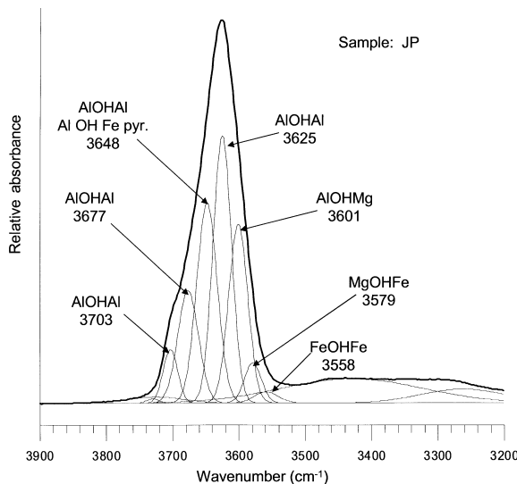
Figure 6. Decomposition of the IR spectrum of Fe-rich montmorillonite Jelsový Potok (JP).
