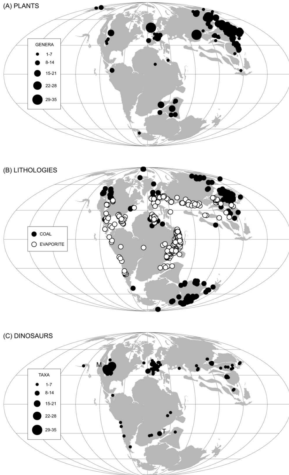
Figure 1. Late Jurassic (150 Ma) paleogeographic maps (Mollweide projection with 30° latitude and longitude lines). A , Plant localities, scaled according to the number of constituent genera. B , Evaporite and coal deposits. C , Dinosaur localities, scaled according to the number of constituent taxa and showing the location of the Morrison ( M ) and Tendaguru ( T ) Formations.
