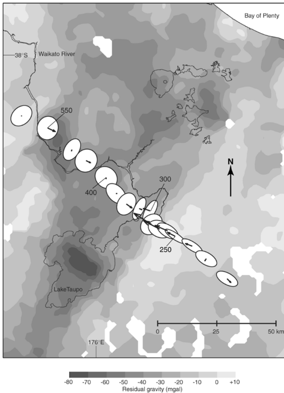
Figure 7. Phase tensor ellipses at T = 21.3 s superimposed on the regional gravity map of the Taupo Volcanic Zone (after Bibby et al. 1995). The ellipses have been drawn so that the major axes are all the same length. Also shown are the corresponding induction arrows (real part).
