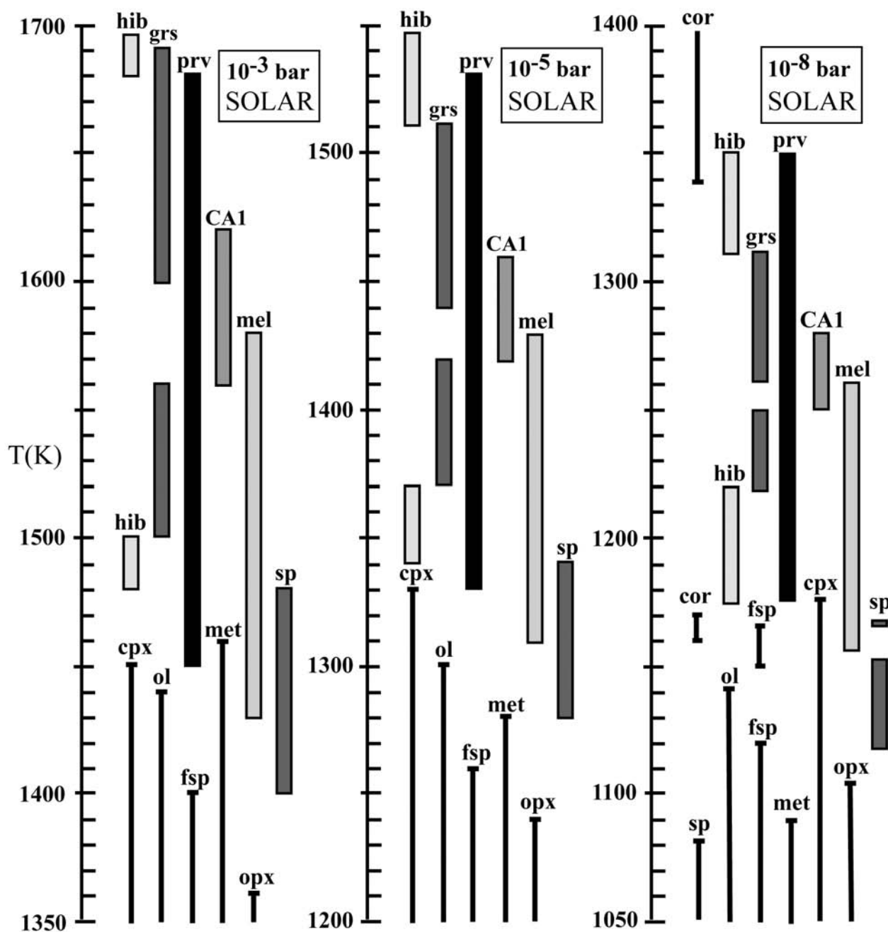
Fig. 5. Appearance and disappearance temperatures of phases hibonite/grossite/Ca-aluminate ( \text{CaAl}_2\text{O}_4 )/melilite/spinel/metal. Phase appearances/disappearances, as in Ebel and Grossman (2000), agree very closely with Yoneda and Grossman and Grossman (1972), below the appearance temperature of spinel, which is the region of interest here. The thermodynamic model is described in Ebel and Grossman (2000), with sapphirine and cordierite suppressed; hib = hibonite, grs = grossite, prv = perovskite, CA1 = \text{CaAl}_2\text{O}_4 , mel = melilite, cpx = Ca-pyroxene, met = Fe, Ni metal, ol = olivine, fsp = feldspar, sp = spinel, opx = low-Ca pyroxene.
