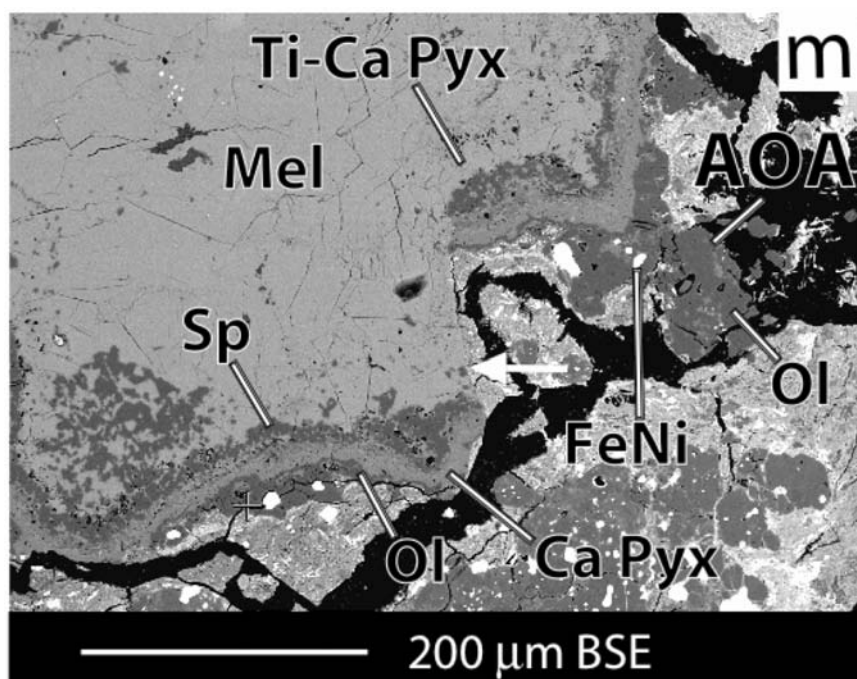
Fig. 1. Continued. Backscattered electron (BSE) images and X-ray maps of AOAs in CR chondrites: m) enlargement of the edge of EET92-21 showing the Wark-Lovering rim and two of the AOAs on the rim. The AOA contains olivine surrounding Ca-pyroxene and FeNi metal. The Wark-Lovering rim is dislocated along one portion (arrow).
