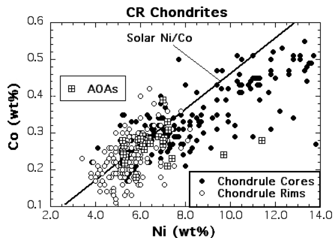
Fig. 4. Plot of Ni versus Co (wt%) showing compositions of FeNi metal in the AOAs in CR chondrites. Also shown is metal from the rims and cores of chondrules in the CR chondrites. Like metal in the chondrules, the AOA metal has positive Ni-Co relationship with Ni:Co ratios that are close to the solar ratio. The AOA metal has compositions that are similar to rim metal and some core metal in the chondrules.
