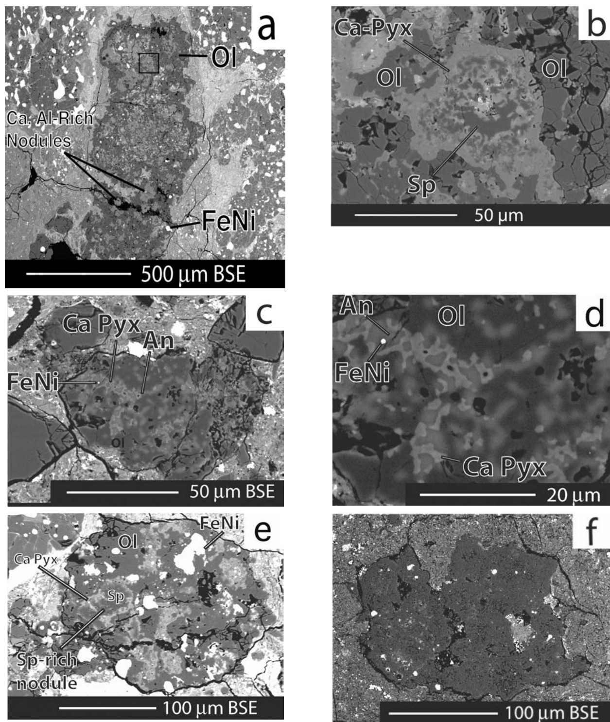
Fig. 1. Backscattered electron (BSE) images and X-ray maps of AOAs in CR chondrites: a) R317 from Renazzo is a relatively large (>600 \mu\text{m} in length) AOA and contains FeNi metal (white) and numerous nodules of Ca-Al-rich assemblages surrounded by sinuous bands of olivine (Ol); b) enlargement of R317 showing a spinel-bearing nodule with spinel (Sp) surrounded by Ca-pyroxene (Ca-Pyx), followed by olivine (Ol); c) EET87-3 from the EET 87770 CR chondrite, consisting of sinuous bands of olivine (Ol) surrounding Ca-pyroxene (Ca-Pyx) and anorthite (An); d) enlargement of a portion of EET87-3 (from [c]) showing the anorthite (An), metal (FeNi metal), and the Ca-pyroxene (Ca-Pyx), which occur as chains of (2 \mu\text{m} size) crystals growing at the boundary between the olivine (Ol) and anorthite; e) EET96-1 is an AOA from EET 96259 that appears to be relatively metal-rich and contains a spinel (Sp)-rich nodule in which spinel is surrounded by anorthite and Ca-pyroxene, rimmed by olivine. Other nodules in this inclusion are composed mostly of Ca-pyroxene and anorthite; f) AR-1 from Al Rais is an AOA that contains metal and has a relatively lower abundance of Ca-Al-rich minerals.
