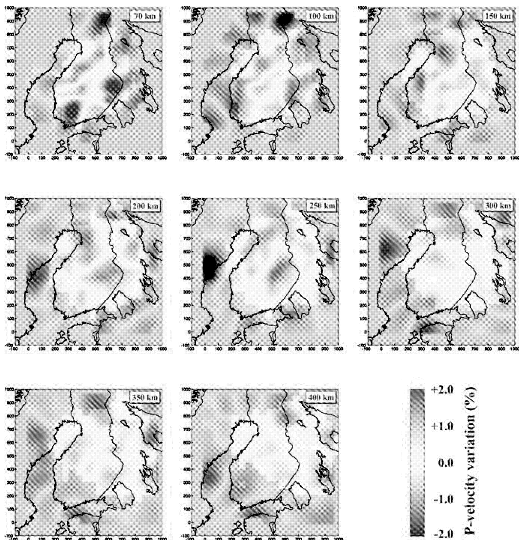
Figure 9. Horizontal sections at different depths (upper right corner, in km) of the recovered upper mantle structure after inverting the observed traveltime residuals without crustal corrections. The crustal layers are left floating during the inversion (not shown).
