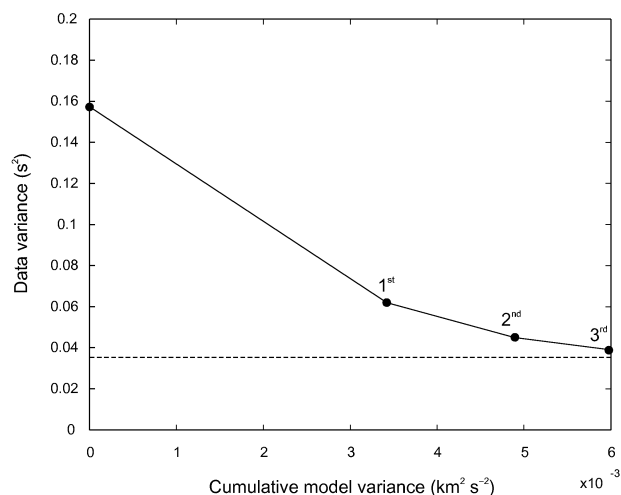
Figure 3. Variance reduction after different iterations during the SVEKALAPKO data set inversion. The dashed line indicates the noise level which is obtained by summing the phase pick data variance and a conservative error estimate in the crustal model (see text).
