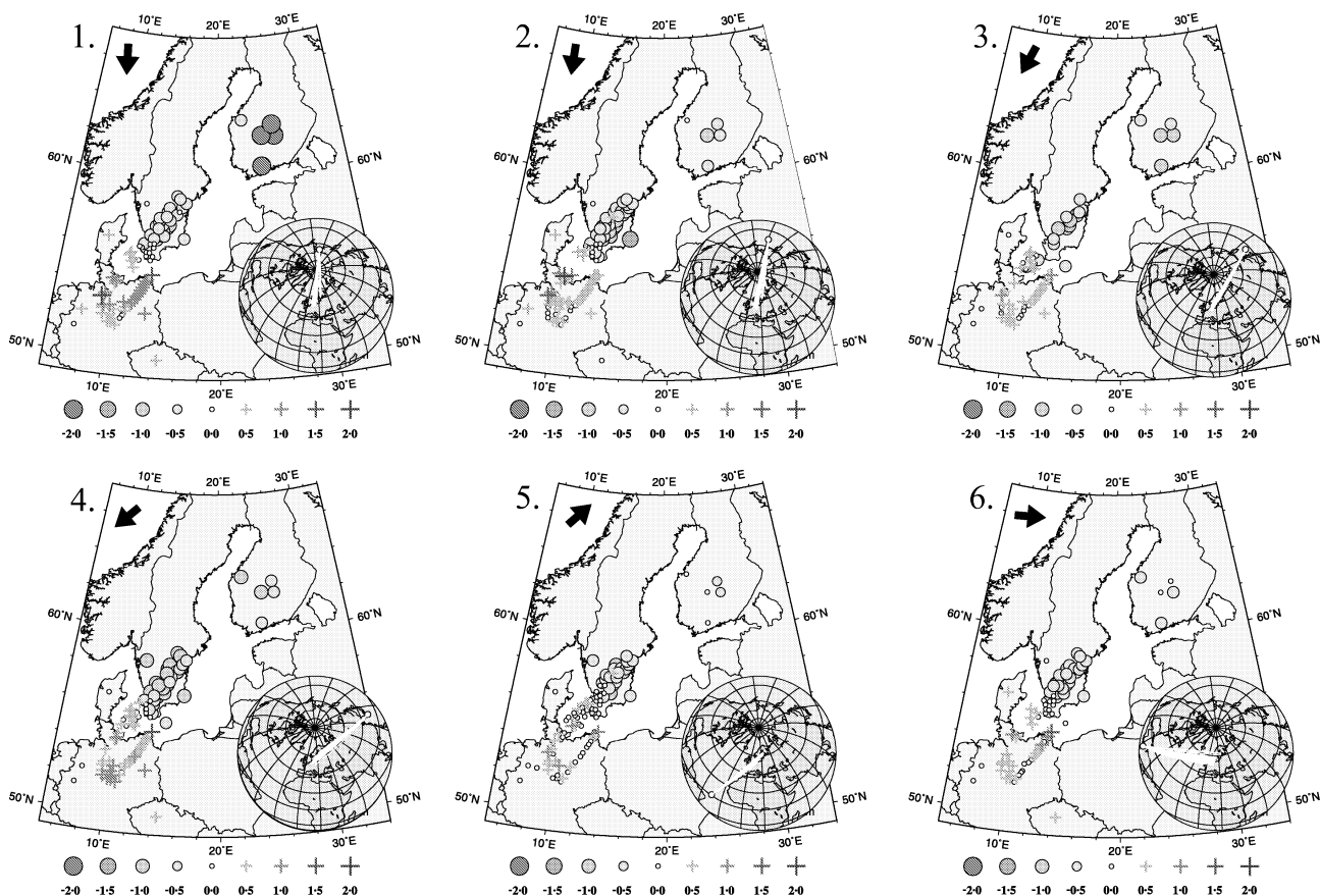
Figure 12. Relative P -wave traveltime residuals for stations at the TOR array and five stations from the Finnish permanent network for six selected teleseismic events (Table 1) from different azimuthal regions. The black arrows indicate the incoming direction of the teleseismic wavefront.
