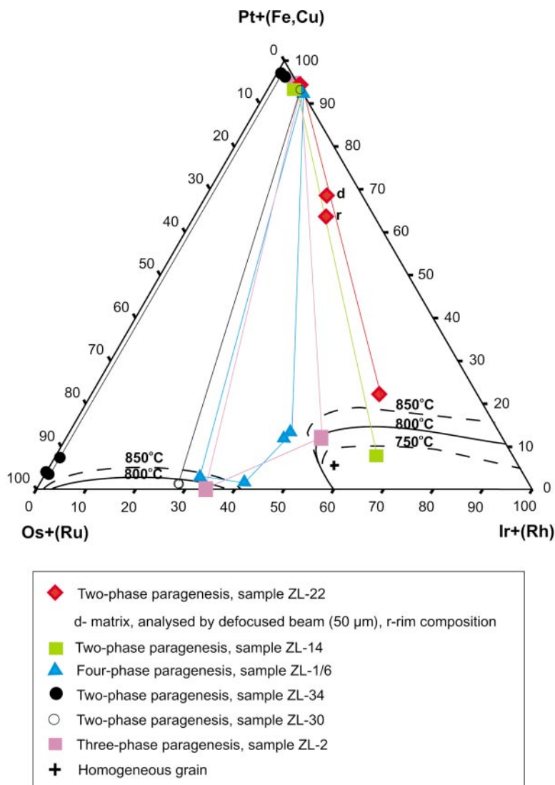
FIG. 10. Phase diagram of the Pt + (Fe,Cu) – Os + (Ru) – Ir + (Rh) system (Slansky et al. 1991).
