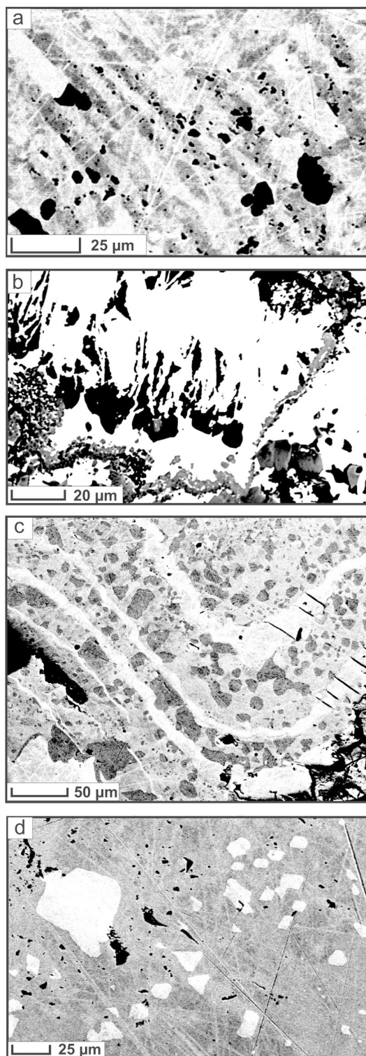
FIG. 6. Back-scattered electron (BSE) images of different exsolution-induced textures of Ir-Os-Ru-Pt alloy from Zolotaya River. a. Micrographic intergrowth of Ir-rich Pt-Fe alloy (white) with Ir-Ru-Pt alloy (grey), and cherepanovite inclusions (dark grey). Sample ZL22. b. Rim zone of Pt-Ir-Fe-Ru alloy (white) with symplectitic inclusions of Ru-rich cherepanovite (black). Irarsite (dark grey) occurs as a reaction rim and on fractures. Sample ZL22. c. Patchy inclusions of Ir-rich Pt-Fe alloy (dark grey) in iridium matrix (grey) and ribbon-like osmium (white). Sample ZL2. d. Subhedral inclusions of iridium (white) in Ir-rich Pt-Fe alloy (grey). Sample ZL14.
