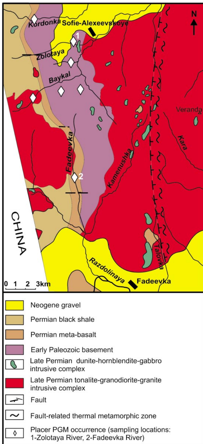
FIG. 2. Geological sketch-map of the study area.
