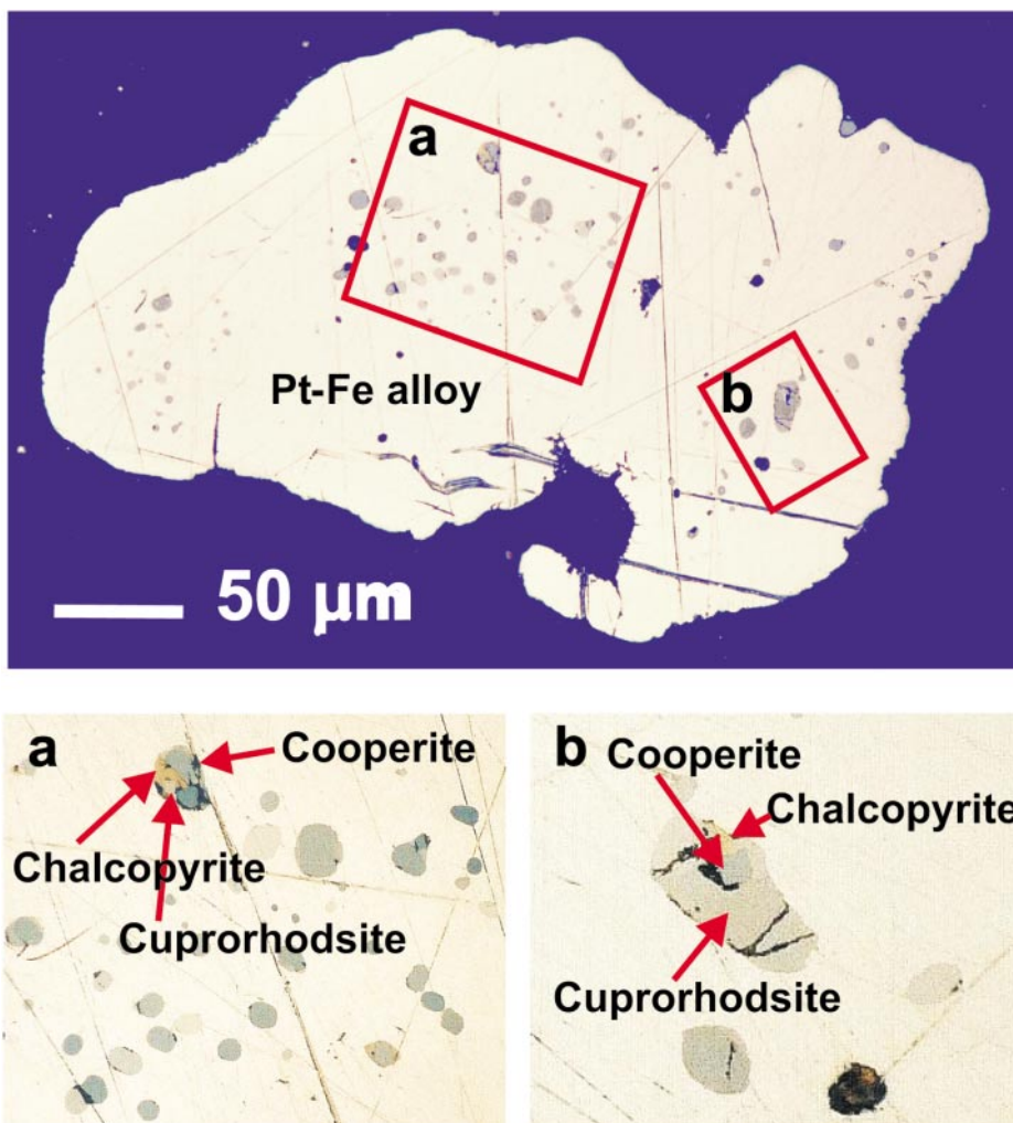
FIG. 7. Cooperite inclusions in Pt-Fe alloy. Sample ZL-1/7.
