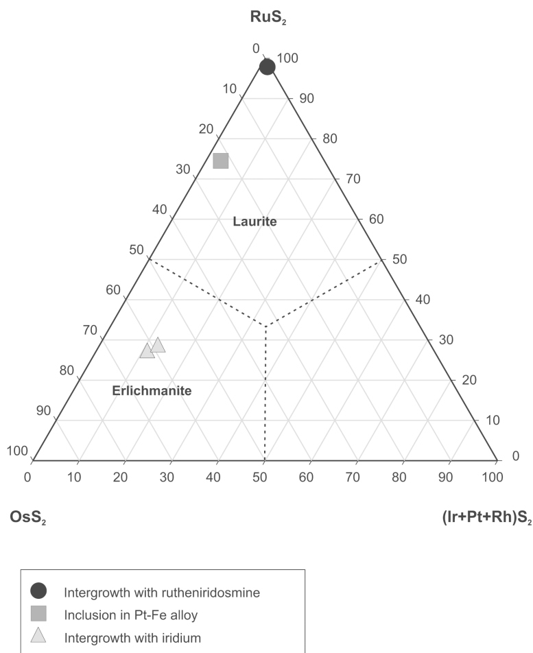
FIG. 9. Mineral composition of the laurite–erlichmanite solid-solution series (at.%).
