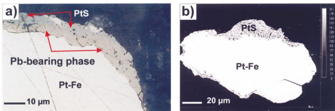
FIG. 8. Secondary rim of cooperite (a) intergrown with Pb-Ir-Cu-Rh sulfide (xingzhongite or konderite) and of cooperite (b) on Pt-Fe alloy.
