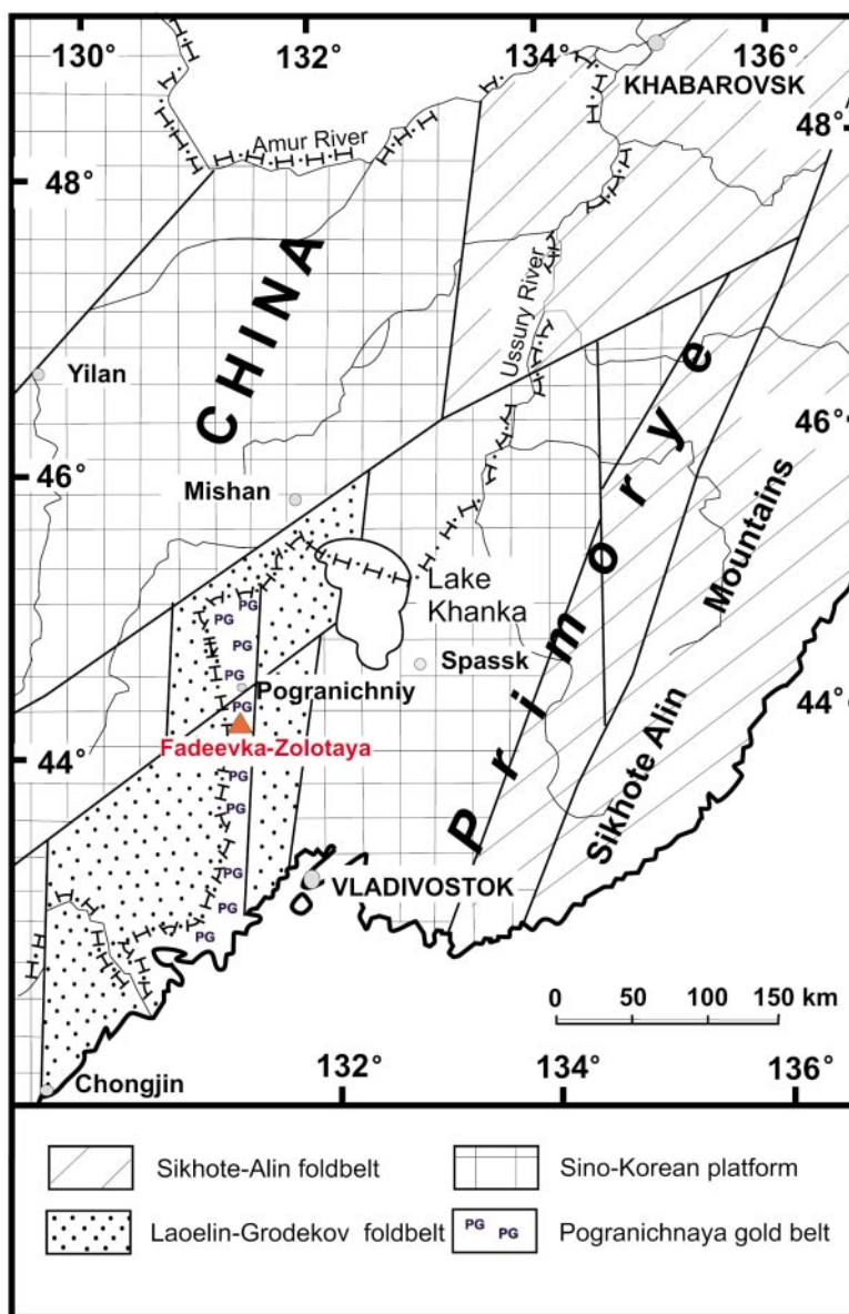
FIG. 1. Location map of the PGE-bearing gold placers of Zolotaya and Fadeevka in Primorye, Russian Far East. Map simplified after Shcheka et al. (2001).
