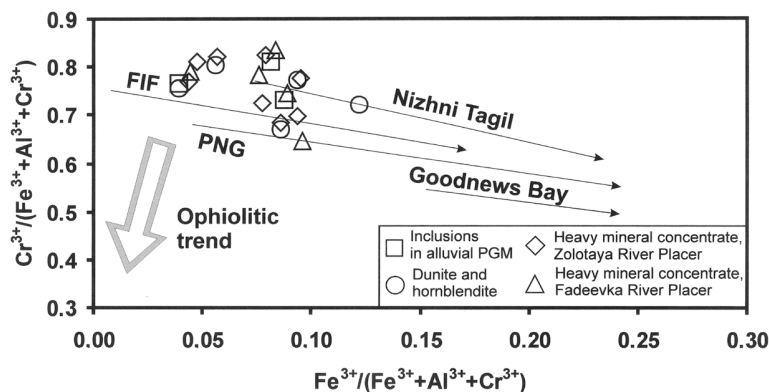
FIG. 3. Plot of \text{Fe}^{3+}/(\text{Cr}^{3+} + \text{Fe}^{3+} + \text{Al}^{3+}) versus \text{Cr}^{3+}/(\text{Cr}^{3+} + \text{Fe}^{3+} + \text{Al}^{3+}) for chromian spinel from the Zolotaya and Fadeevka areas. Evolution trends of chromian spinel in the Nizhni Tagil, Fifielid (FIF), Goodnews Bay and Papua New Guinea (PNG) Uralian–Alaskan-type complexes, as well as for ophiolitic chromitites, according to Johan (2002).
