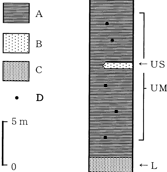
Figure 2. Columnar section of the fossil locality. A. Black mudstone, B. Sandstone, C. Alternation of fine-grained sandstone and mudstone, D. Calcareous concretions. L, UM, US show horizons of fossils ( see the text ).
