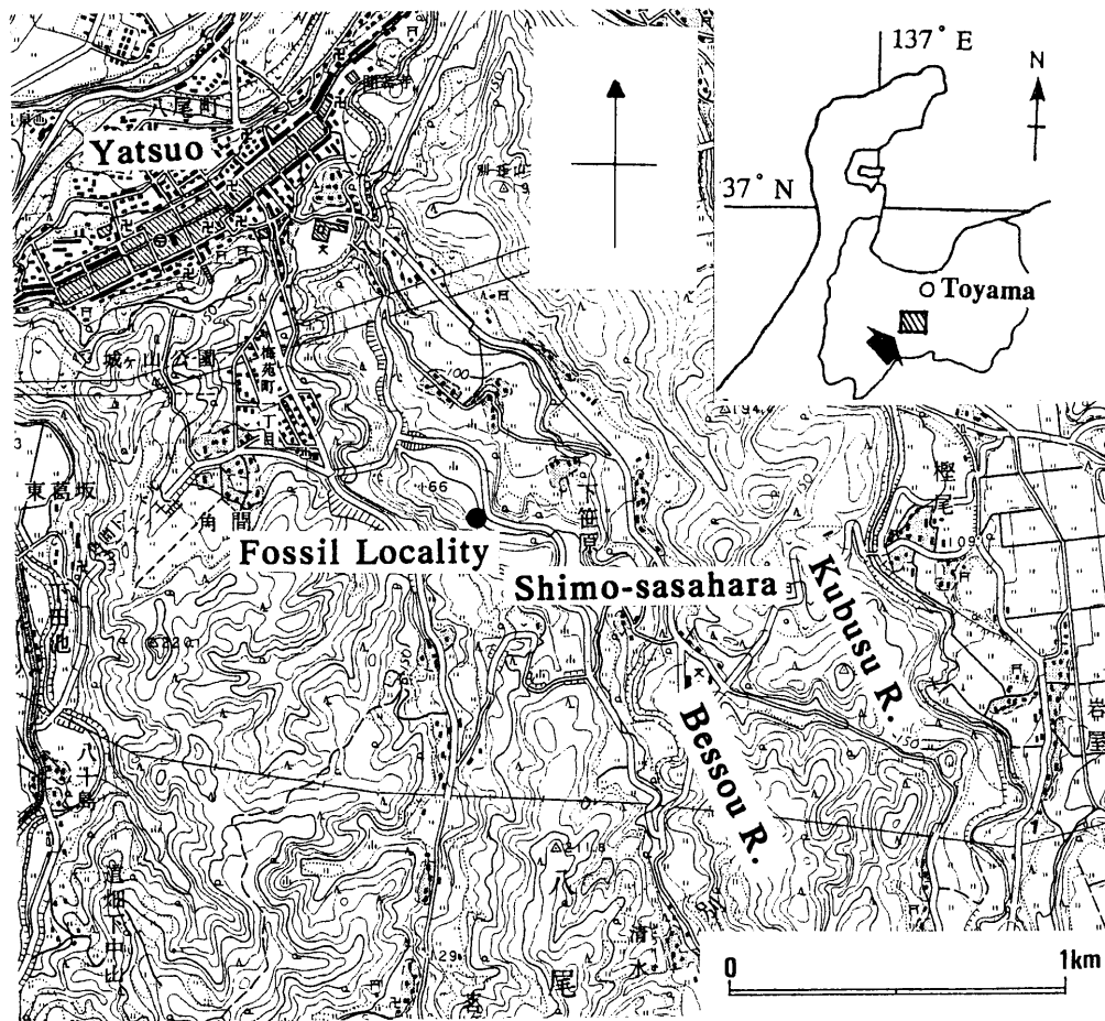
Figure 1. Locality of fossils (from Amano et al. , 2001, fig. 1; using the topographical map of “Yatsuo”, scale 1:25,000, published by Geographical Survey Institute of Japan).
