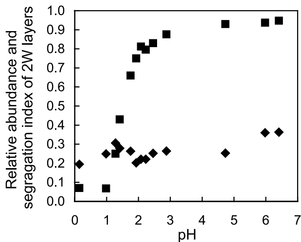
Fig. 13. Relative abundance of 2W layers obtained from XRD profile modelling (solid squares) and segregation index of 2W layers ( S_g(2W) – solid diamonds) as a function of pH under acidic conditions.
