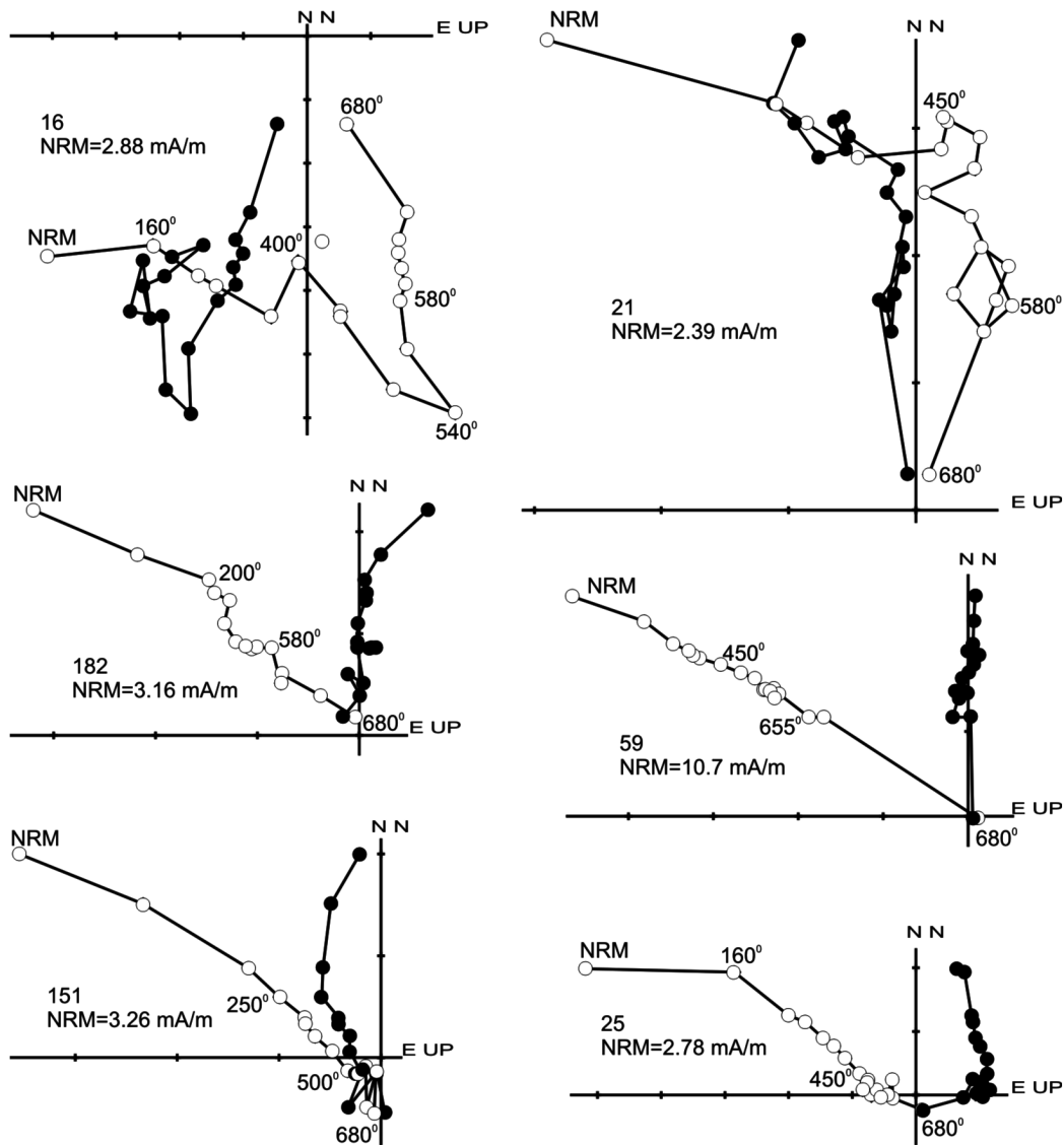
Figure 6. The Zijderveld diagrams typical for the rocks of the Mota and Irkutsk formations of the Central Sayan region (Urik R. area). The solid circles show the projection of the magnetization vector onto the horizontal plane, the open ones, onto the vertical. All diagrams are plotted in the stratigraphic coordinates.
