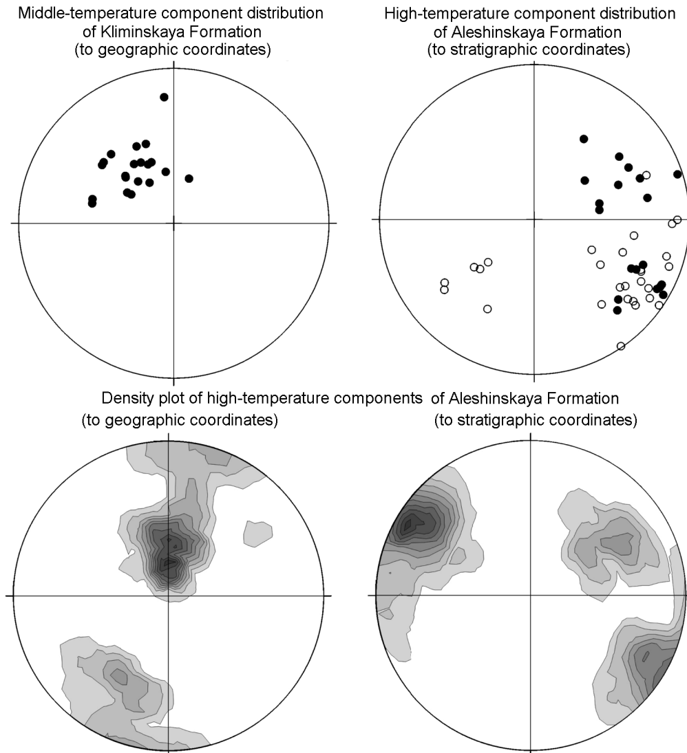
Figure 14. The distribution of the vectors of the magnetization components in the rocks of the Kliminskaya and Alesha formations of the Yenisey Range where it is crossed by the Taseeva River. The stereograms of the density distribution of the respective high-temperature magnetization components of the rocks of the Alesha Formation. The solid circles denote the projections to the lower hemisphere, the open ones, to the upper one. All axes of the density stereograms face the lower hemisphere.
