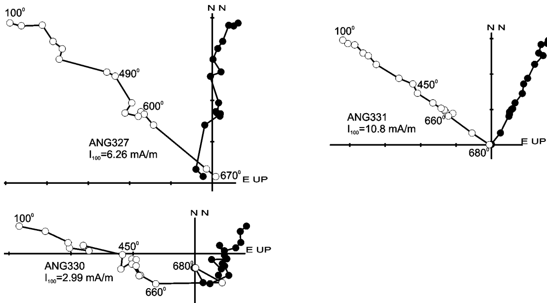
Figure 9. The typical Zijderveld diagrams for the rocks of the Redkolesnaya Formation in the Yenisey Range. The solid circles mark the projections of the magnetization vector onto horizontal plane, the open ones, onto the vertical. All diagrams are given in the stratigraphic system of the coordinates.
