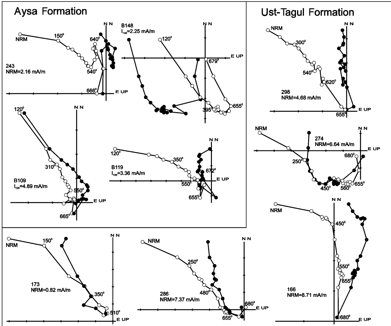
Figure 5. The Zijderveld diagrams typical of the rocks of the Aisa and Ust-Tagul formations in the Biryusa area of the Sayan region. The solid circles mark the projections of the rocks onto the horizontal plane, the open circles, onto the vertical plane. All diagrams are plotted in the stratigraphic system of the coordinates.
