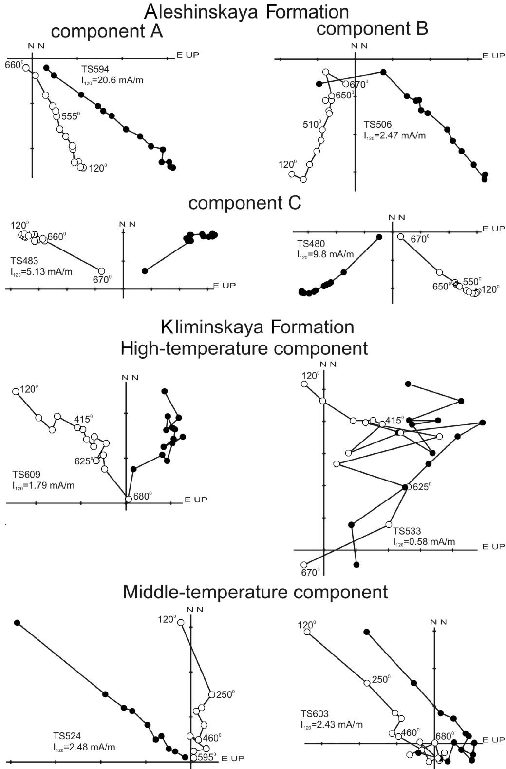
Figure 7. The typical Zijderveld diagrams for the rocks of the Alesha and Kliminskaya formations of the Yenisey Range (Taseeva R. area). The solid circles show the projections of the magnetization vector onto the horizontal plane, the open ones, onto the vertical. All diagrams are plotted in the stratigraphic system of the coordinates.
