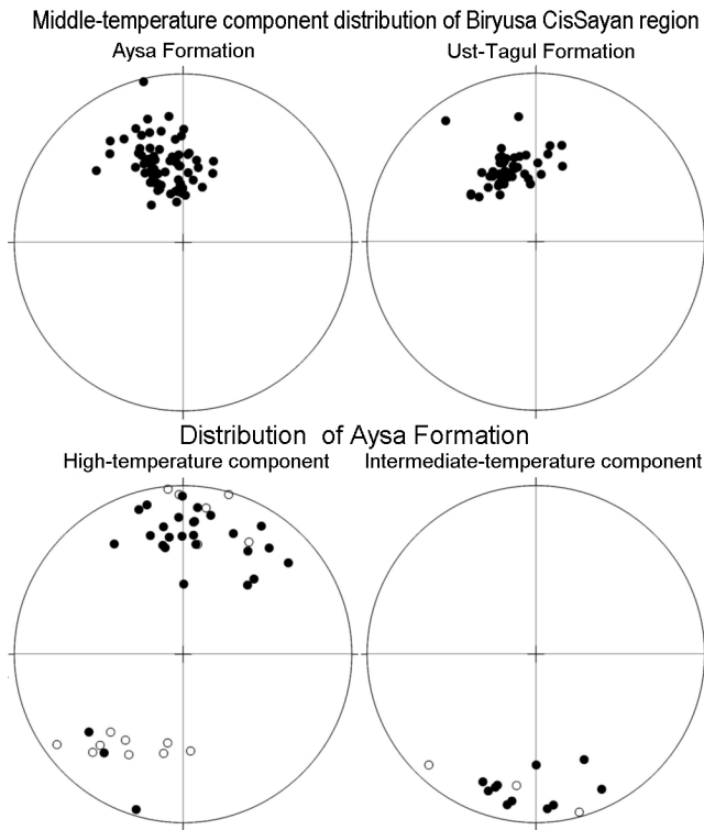
Figure 10. The distribution of the vectors obtained for the medium-temperature, intermediate, and high-temperature magnetization components of the Aisa Formation and for the medium-temperature component of the Ust-Tagul Formation in the Sayan region bordering the Biryusa R. The stereograms are presented in the stratigraphic coordinates. The solid circles show the projections to the lower hemisphere, the open ones, for the upper one.
