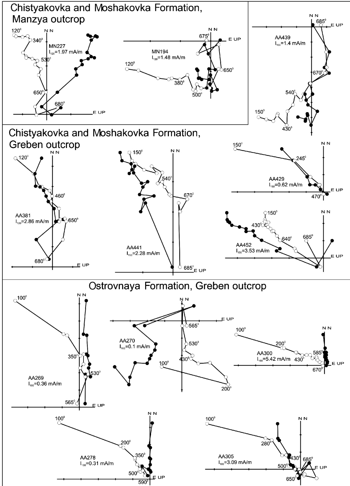
Figure 8. The typical Zijderveld diagrams for the rocks of the Taseeva Series and for the insular rocks of the lower Angara R. sequences of the Yenisey Range. The solid circles show the projections of the magnetization vector onto the horizontal plane, the open ones, onto the vertical plane. All diagrams are plotted in the stratigraphic system of the coordinates.
