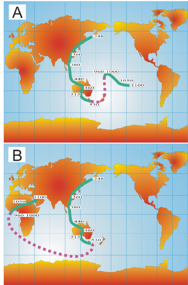
Figure 16. The configuration versions for the curve of the apparent migration of the Siberian Platform pole as a function of the positions of the Late Riphean–Vendian paleomagnetic poles. (A) - classic [Pecherskiy and Didenko, 1995; Smethurst et al. , 1998] and (B) - alternative approach to poles of Late Precambrian paleomagnetic orientations.
