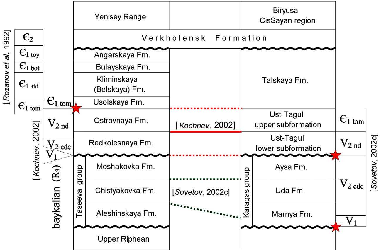
Figure 4. Correlation of the rock sequences studied in the Yenisey Ridge and in the Biryusa area of the Sayan region. The red stars indicate the most important stratigraphic bench marks (see the text for the explanation).
