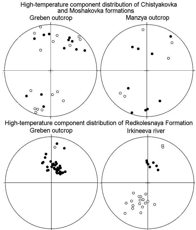
Figure 11. The distribution of the vectors of the high-temperature magnetization component in the rocks of the Taseeva Series and Redkolesnaya Formation of the Yenisey Range. The stereograms are presented in the stratigraphic system of the coordinates. The solid circles mark the projections to the lower hemisphere, the open ones, those to the upper one.
