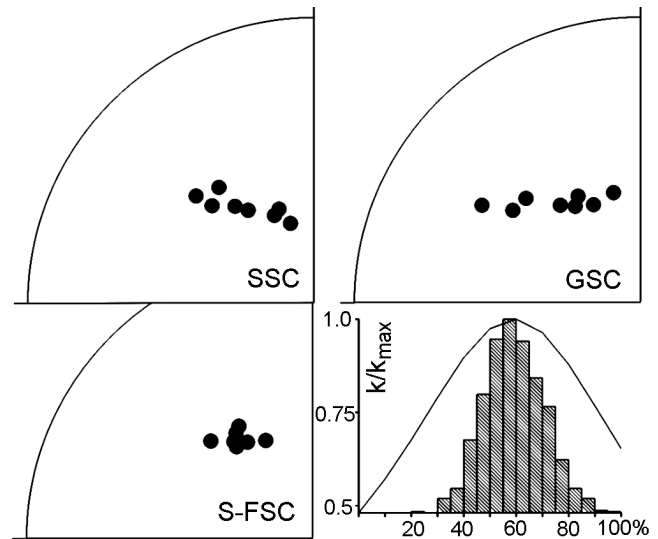
Figure 13. The distribution of the site-averaged values for the medium-temperature component of the Taseeva rock series and the Ostrovnyaya rocks of the Greben sequence from the Yenisey Range. The proportional fold flattening and the Watson-Enkin test for the average values are given for the values averaged for the sites. SSC is the abbreviation for the stratigraphic system of the coordinates; GSC, for the geographical system of the coordinates, S-FSC, for the syn-folding system of the coordinates (the nonproportional straightening of the fold by the method of the intersection of small circles). The solid circles are used for the projections onto the lower hemisphere.
