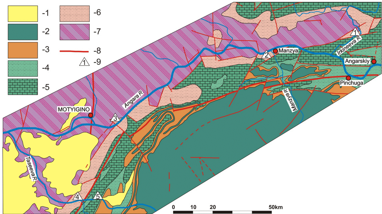
Figure 2. The schematic geological structure of the Yenisey Ridge study area. Legend: 1 – Neogene, 2 – Permian-Triassic traps, 3 – Carboniferous and Permian rocks, 4 – Middle-Upper Cambrian (Upper Lena Formation), 5 – Lower Cambrian, 6 – Upper Riphean(?) to Vendian rocks (Taseeva Series: Redkolesnaya and Ostrovnaya formations), 7 – pre-Vendian rocks, 8 – faults; 9 – objects of study: (1) the Irkineeva R. area: the rocks of the Redkolesnaya Formation; (2) the left bank of the Angara R. below the Man'zya Settlement: the rocks of the Chistyakova and Moshakova formations, (3) the right bank of the Angara R. from the Gremyachiy Creek to the Greben Cliff: the Chistyakova, Moshakova, Redkolesnaya, and Ostrovnaya formations, (4) the right bank of the Taseeva R. below the mouth of the Usolka River: the Alesha Formation, and (5) the right bank of the Taseeva R. in the area of the Dyrovatyi Cliff: the Kliminskaya Formation.
