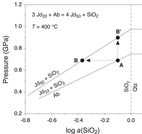
Fig. 4. P – \log a(\text{SiO}_2) diagram showing the upper pressure breakdown reaction of albite to omphacite + \text{SiO}_2 in the \text{SiO}_2 -undersaturated field for pure albite and for omphacite with \text{Jd}_{33} and \text{Jd}_{50} .
