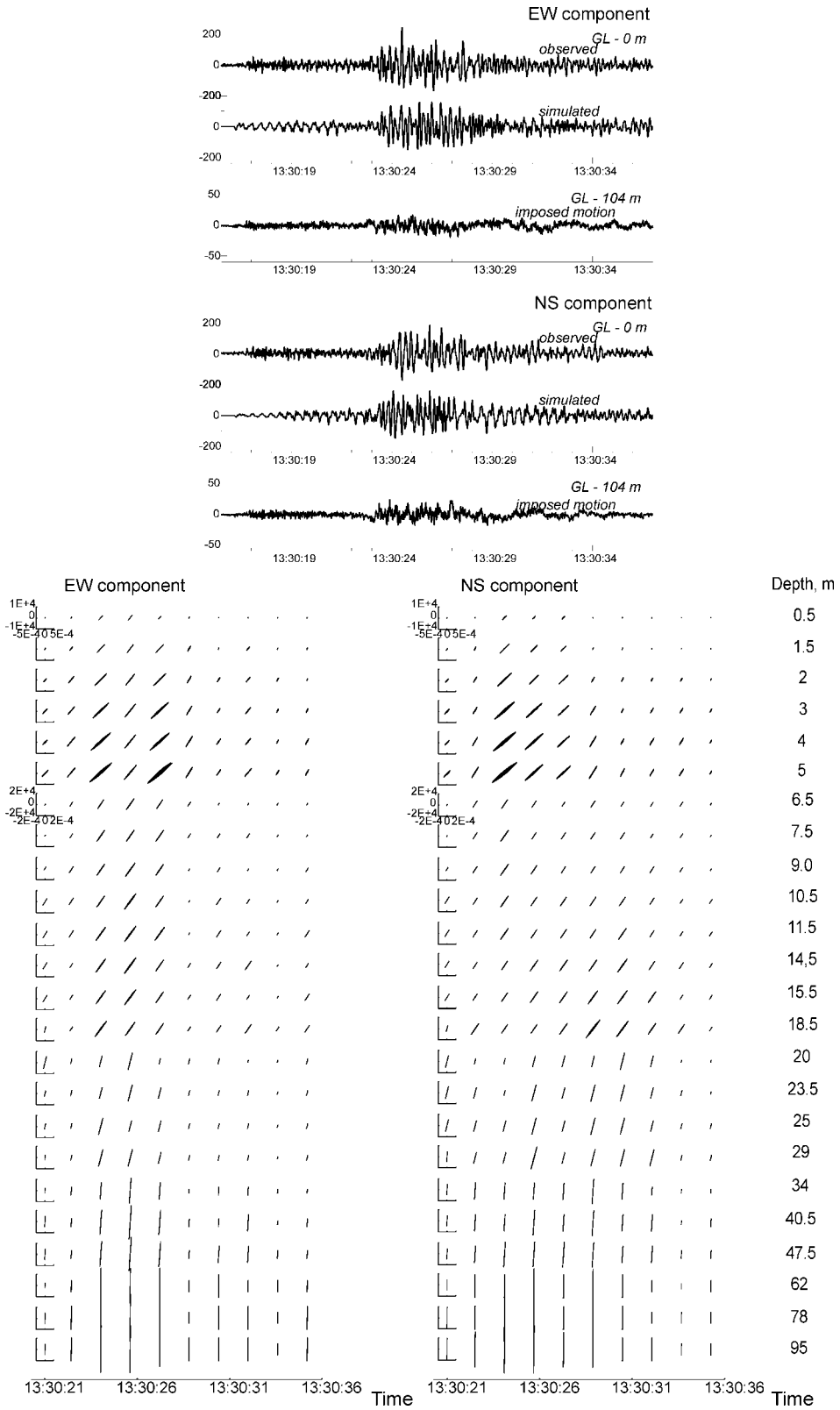
Figure 5. Same as Figure 3 for the HRS06 station (stresses are given in Pa; strains, in strains, the same scales for depths 0–5 m and 6–100 m).
