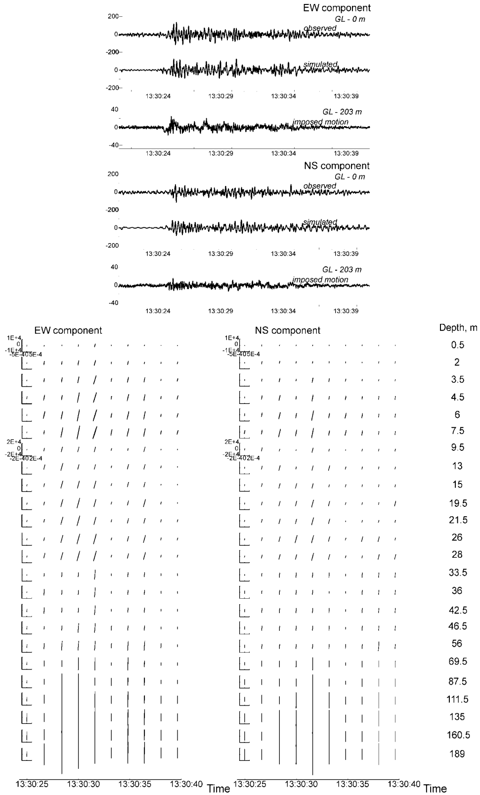
Figure 7. Same as Figure 3 for the HRS05 station (stresses are given in Pa; strains, in strains, the same scales for depths 0–7 m and 8–100 m).
