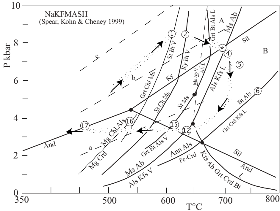
Figure 8. P - T trajectory shown by the shallower samples. The figures indicate the reactions described in the text. 'A' is melting region from vapour-saturated (asterisk) to vapour-absent conditions predicted for the pelitic system; experimental studies have shown that in this region, sodic melts (like most of the leucosomes of the studied profile) and peritectic staurolite (part of the relict St_1 ?) form at T around 700 °C under P of 6–10 kbar (Patiño Douce & Harris, 1998; Garcia Casco et al. 2003). 'B' is region characterized by melting reactions Bt + Sil + Qtz + Pl = Grt + Kfs + L or Mg-Crd + Kfs + L , depending on the Mg of the bulk composition; 'a' Ms with Si_{11ox} = 3.10 ; 'b' Ms with Si_{11ox} = 3.20 ; 'c' Ms with Si_{11ox} = 3.30 (Massone in Brouwer, Vissers & Lamp, 2002). Triple point after Pattison (1992). Reaction curves in the NaKFMASH system after Spear, Kohn & Cheney (1999). Reaction MgCrd = MgChl + Als in KFMASH system.
