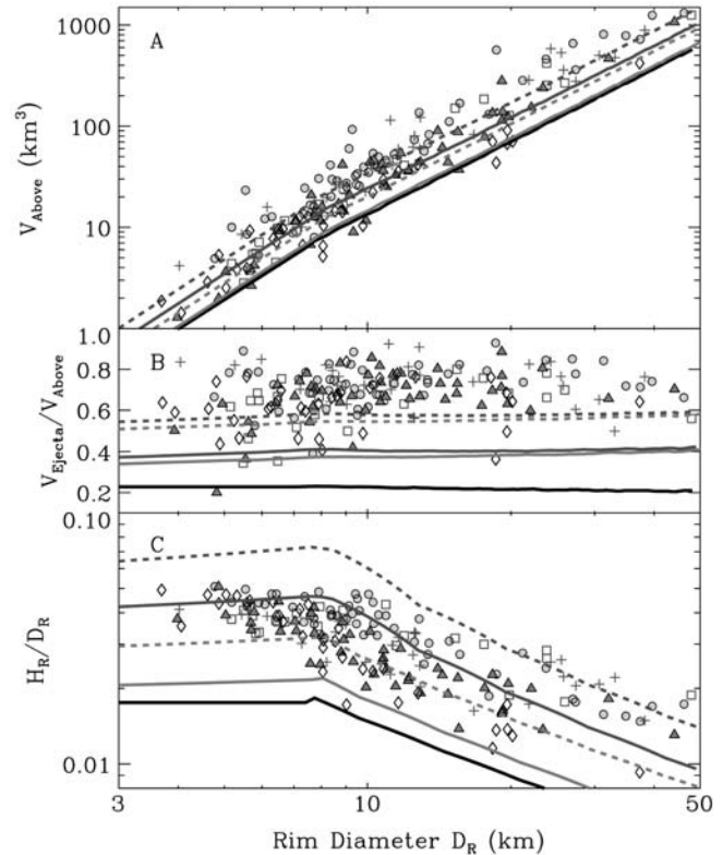
Fig. 22. Z model predictions compared to crater geometry measurements for (a) V_{Above} = V_{Uplift} + V_{Ejecta} , (b) V_{Ejecta}/V_{Above} , and (c) rim height-rim diameter ratio. Original Z model (solid black line), Z-EDOZ model (solid green line), and Z-EDOZ model with ejecta volume increased by a factor of 2 (dashed green line). Z-EDOZ model (solid red line) and Z-EDOZ model with twice ejecta volume (dashed red line) using alternate crater size scaling factor C_D C_R = 1.4 . Z = 2.7 in all cases. Utopia basin = circles; Isidis basin = squares; Acidalia Planitia = crosses; Lunae Planum = triangles; Solis Planum = diamonds.
