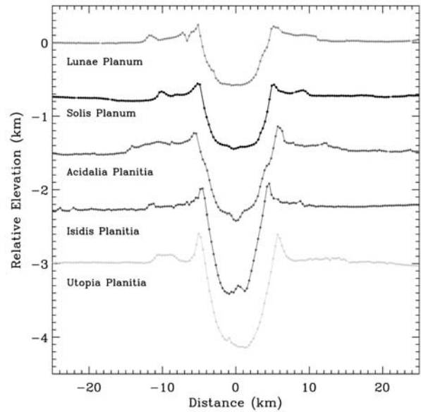
Fig. 11. Typical MOLA altimetry profiles passing near the center of fresh craters ( D^R \sim 9 km). Each dot represents an individual MOLA measurement. Crater locations: L.P. (293.0°E, 18.6°N); S.P. (277.0°E, 19.5°S); A.P. (325.8°E, 39.1°N); I.P. (88.0°E, 12.8°N); U.P. (109.6°E, 34.2°N). The vertical exaggeration is 10:1. The sharp dip in the profile near the Lunae Planum crater rim is a small crater which formed on the ejecta blanket.
