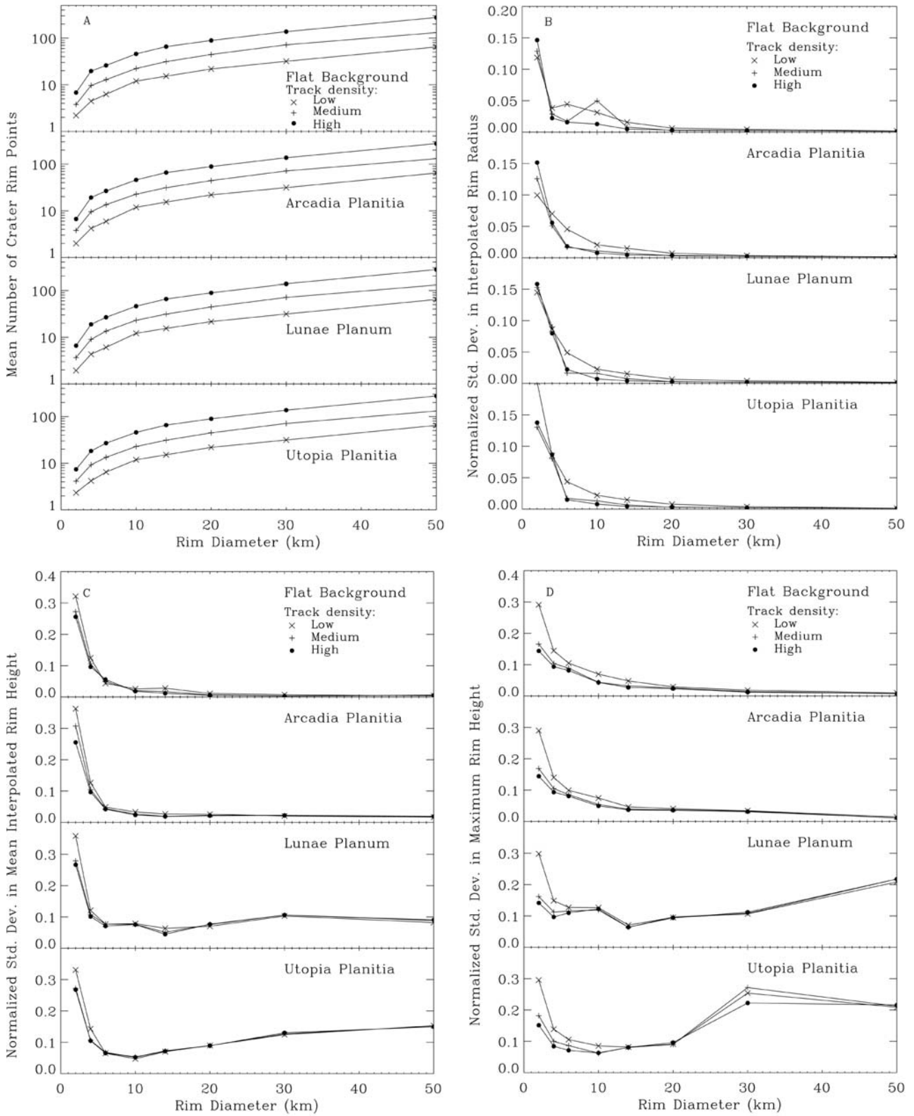
Fig. 5. Error analyses for HMars measurements of simulated crater data sets. a) Mean number of crater rim points. b) Normalized standard deviation ( 1\sigma_m /actual value) in interpolated rim radius. c) Normalized standard deviation in mean interpolated rim height. d) Normalized standard deviation in maximum rim height.
