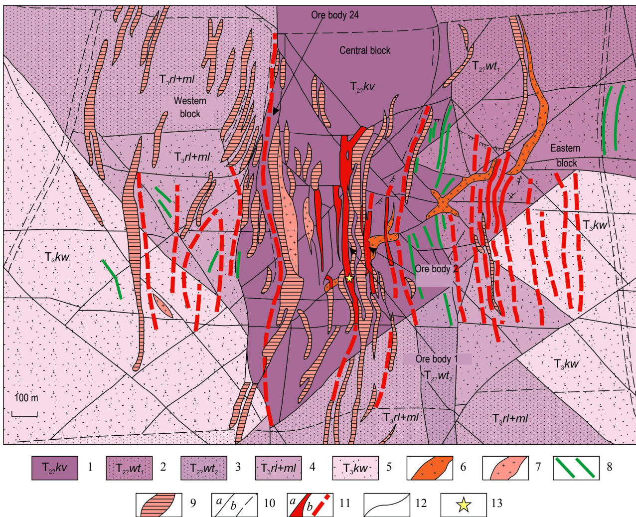
Fig.1. Scheme of the geological structure of the Mayskoe deposit according to A.V. Volkov et. al. [3] with additions Middle (?) Triassic: 1 – siltstones of the Keveyem suite; 2 – uneven-grained sandstones of the Vatapvaam suite, lower subsuite; 3 – uneven-grained sandstones of the Vatapvaam suite, upper subsuite.
