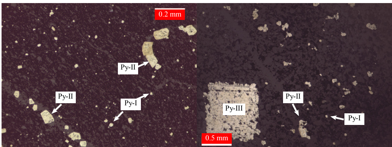
Fig. 7. Pyrite generation from Od-100 sample (reflected light)
