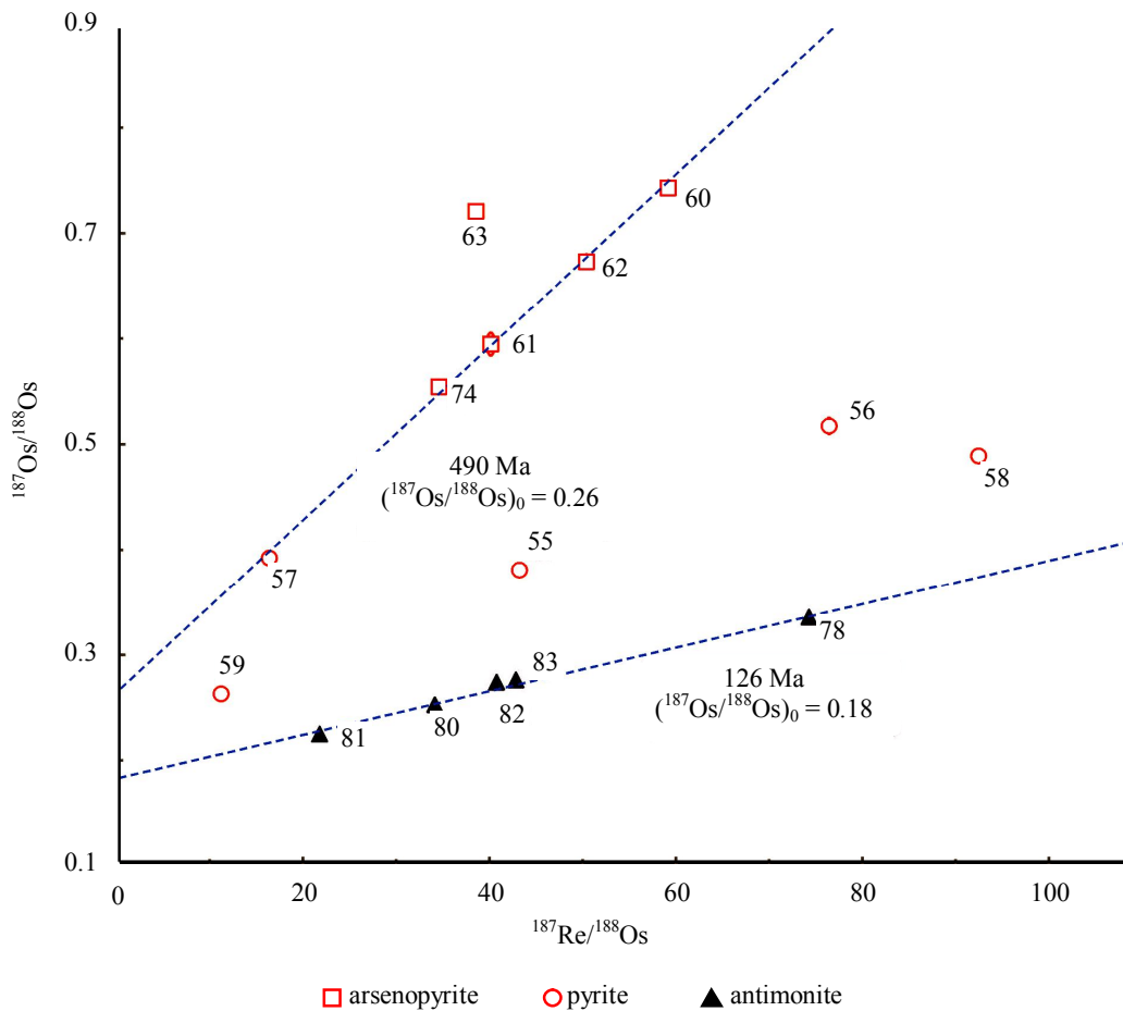
Fig. 3. Re-Os diagram for the studied sulfides of the Mayskoe deposit. The point numbers correspond to the numbers of the analyzed single fractions (see Table). The image of the measured ratio error is less than the characters the size. Reference isochrons of the corresponding age and initial isotopic composition are given to discuss the results
