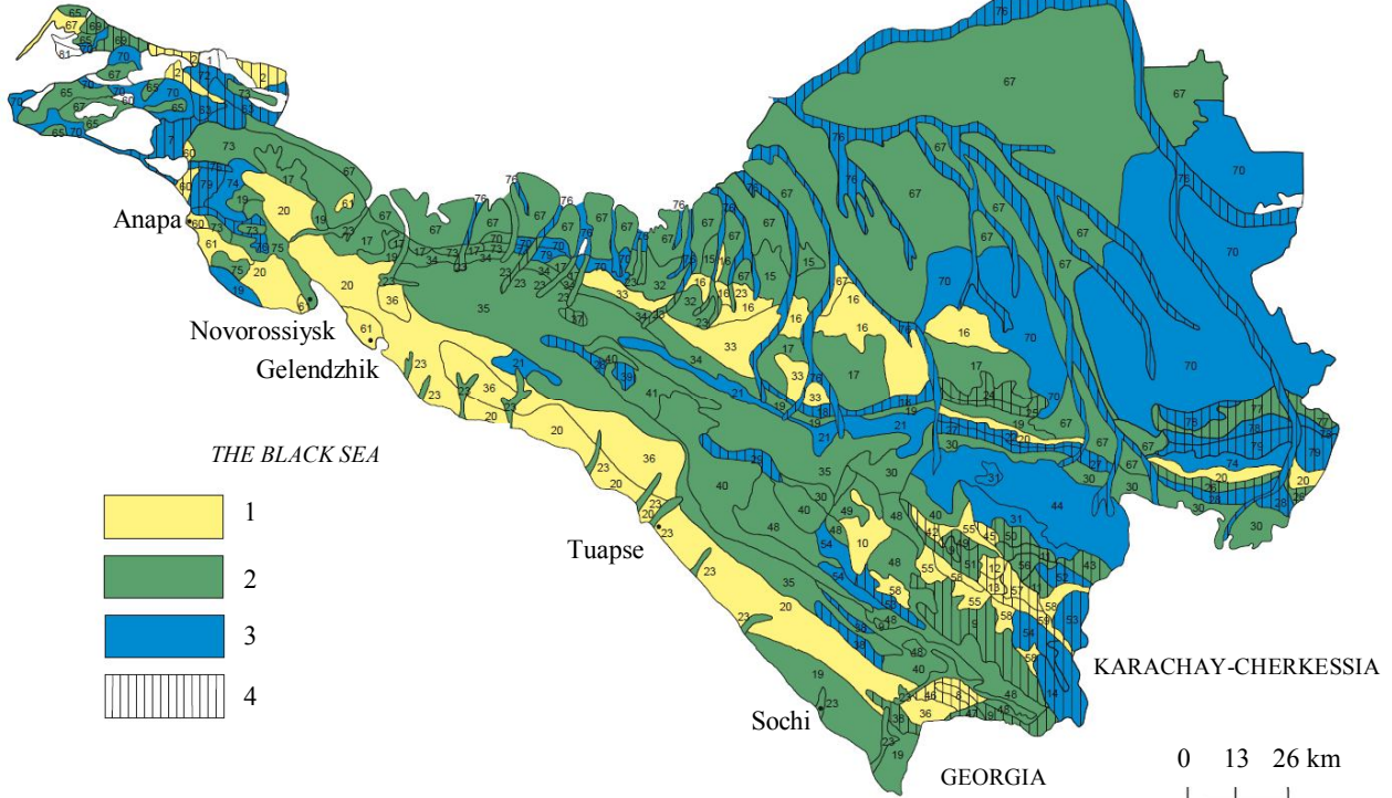
Fig.5. Map of mean background content of Mn ( n \cdot 10^{-3}\% ) in the soils of the western part of the North Caucasus
