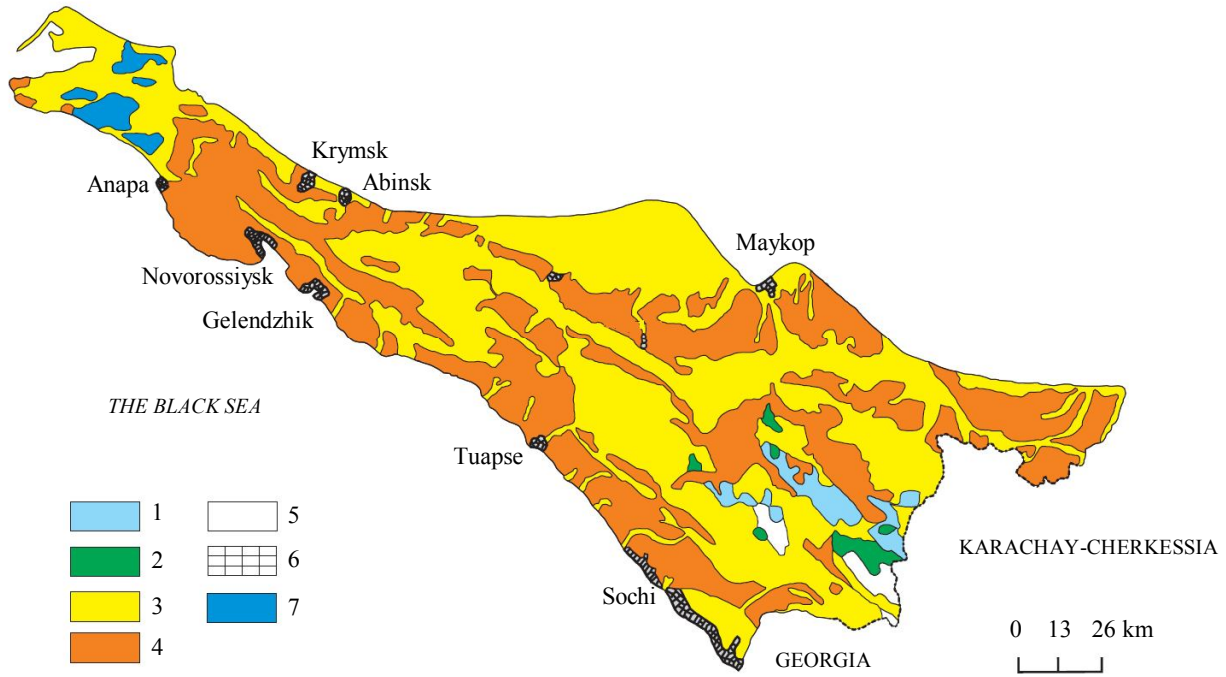
Fig.4. Map of mean background content of Mn ( n \cdot 10^{-3}\% ) in the rocks of the western part of the North Caucasus
