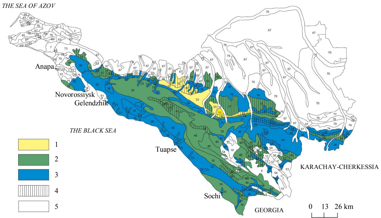
Fig. 6. Map of mean background content of Mn ( n \cdot 10^{-3}\% ) in the ashes of hornbeam leaves 1 – 725-850; 2 – 552-724; 3 – 80-551; 4 – average levels; 5 – landscapes with plant communities without hornbeam
