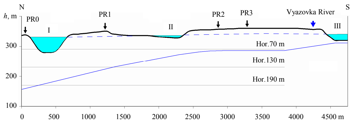
Fig. 6. Schematic longitudinal section in the center of the Degtyarsky mine field
