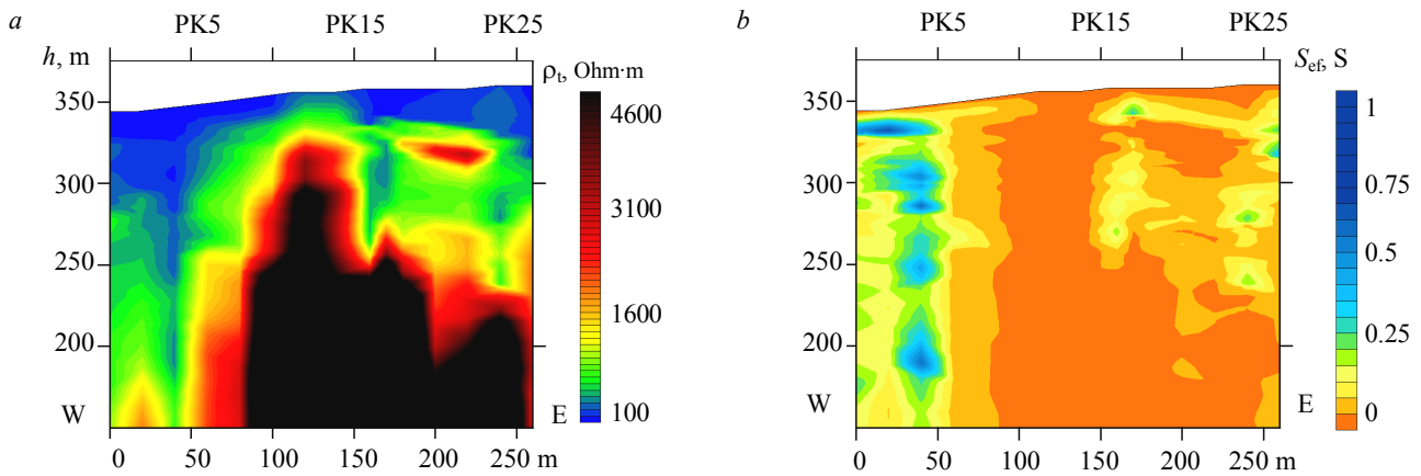
Fig. 3. Deep sections of electrophysical parameters on the PR1 section in the area of the Kapitalnaya-1 mine: a – apparent resistivity; b – effective longitudinal conductivity
