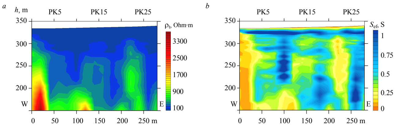
Fig. 2. Deep sections of electrophysical parameters on the PR0 profile in the area of the Kolchedannaya quarry: a – apparent resistivity; b – effective longitudinal conductivity
