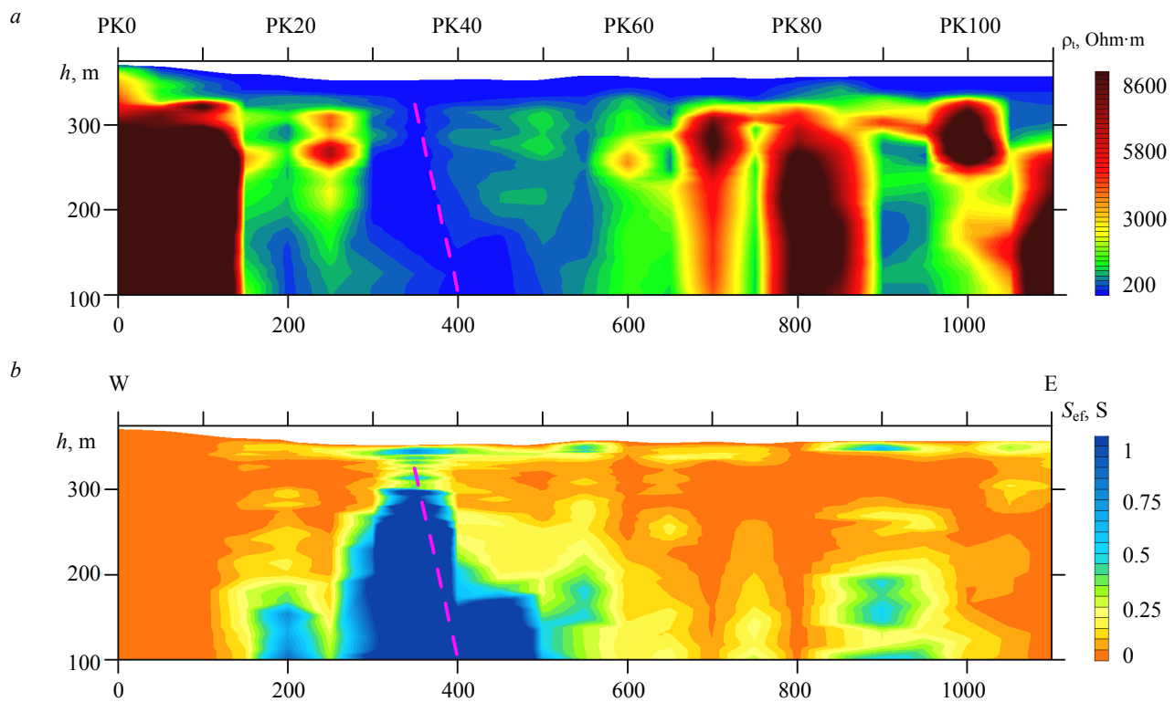
Fig.5. Deep sections of electrophysical parameters along the PR3 section in the area of the Komsomolskaya mine: a – apparent resistivity; b – effective longitudinal conductivity; dotted line shows the axis of the Serov-Mauk fault
