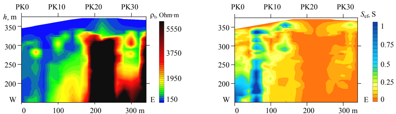
Fig.4. Deep sections of electrophysical parameters on the PR0 in the area of the Moskva mine: a – apparent resistivity; b – effective longitudinal conductivity
