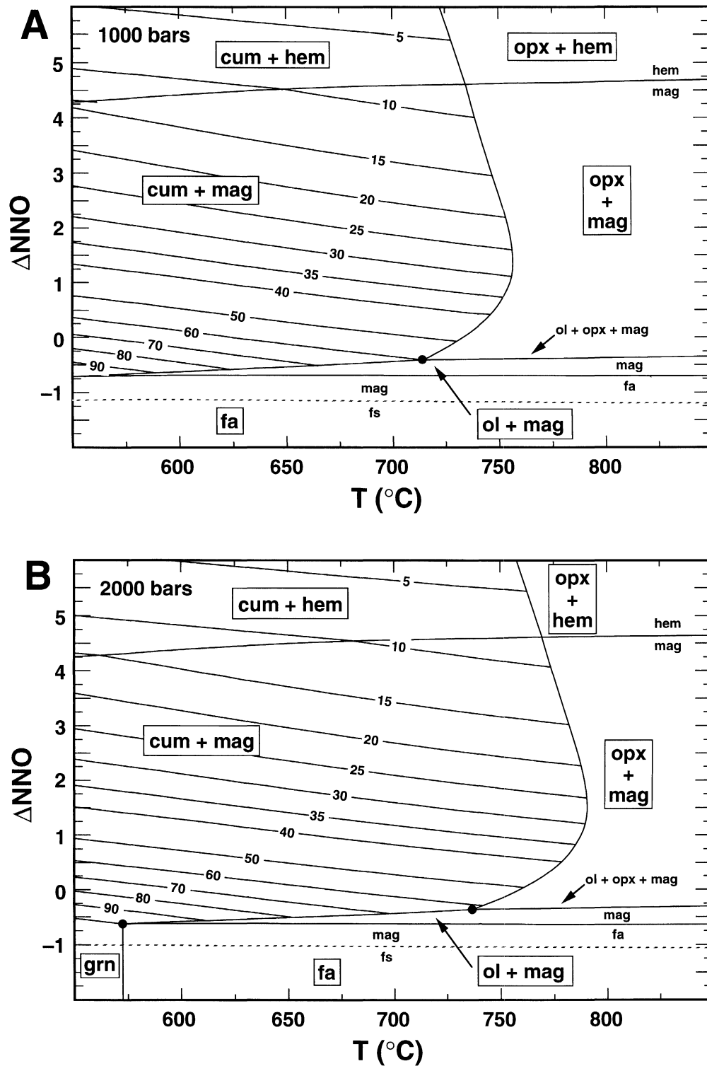
Fig. 9. Calculated T-\Delta \log f_{O_2} ( \log f_{O_2} in excess of NNO) phase diagrams at 1 (A), 2 (B), 5 (C), and 10 kbar (D) illustrating redox and dehydration equilibria in the system FMSHO involving cummingtonite, olivine, orthopyroxene, magnetite, hematite, quartz, and H_2O . Depicts only quartz-saturated relations. Isopleths are percent grunerite in cummingtonite.
