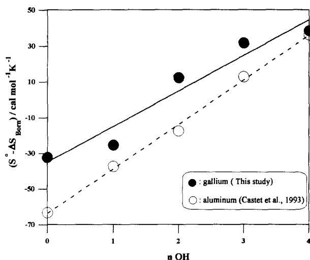
Fig. 3. Correlation of the standard partial molal non-solvation entropies ( S^0 - \Delta S_{\text{Born}} ) of Al and Ga hydroxides complexes with the number of \text{OH}^- ions ( n_{\text{OH}^-} ) in the complexes. The filled circles correspond to the calculated values using data in Table 9 and the solid line is obtained by a linear regression. The open circles and the dashed line correspond to the values for aluminum aqueous species deduced from the data of Castet et al. (1993).
