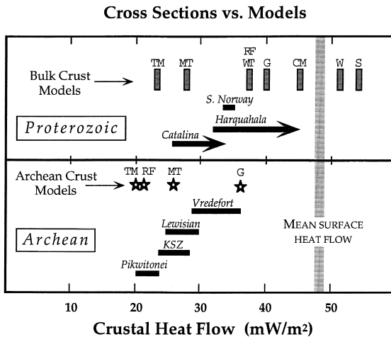
Fig. 2. Comparison of crustally generated heat flow estimated from crustal cross sections (Table 3) and model crust compositions (Table 1). Archean crustal models shown as stars in lower panel. Bulk crustal models shown as vertical bars in upper panel. The gray vertical band marks the range of mean surface heat flow for stable continental crust, as estimated in the text and Table 2. TM = Taylor and McLennan (1985), MT = McLennan and Taylor (1996), RF = Rudnick and Fountain (1995), WT = Weaver and Tarney (1984), G = Gao et al. (1998), CM = Christensen and Mooney (1995), W = Wedepohl (1995), S = Shaw et al. (1986).
