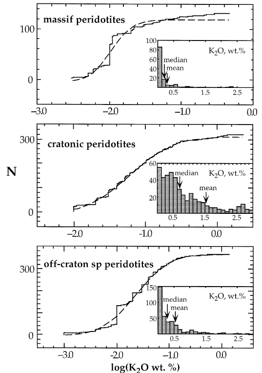
Fig. 4. Cumulative distributions of K_2O analyses for three types of peridotites. The data were fit with an error function N = a_0 + a_1 \text{erf}((x - a_3)/a_4) where x = \log(K_2O \text{ wt}\%) . The fits are shown as dashed lines. Parameters in the fit are: massif: a_0 = 57 , a_1 = 61 , a_2 = -2.0 , a_3 = 0.34 ; cratonic: a_0 = 180 , a_1 = 185 , a_2 = -1.6 , a_3 = 0.73 ; off-craton: a_0 = 151 , a_1 = 160 , a_2 = -1.2 , a_3 = 0.69 . The massif data could also be fit with two error functions, which are not shown. Insets show histograms of K_2O in wt%.
