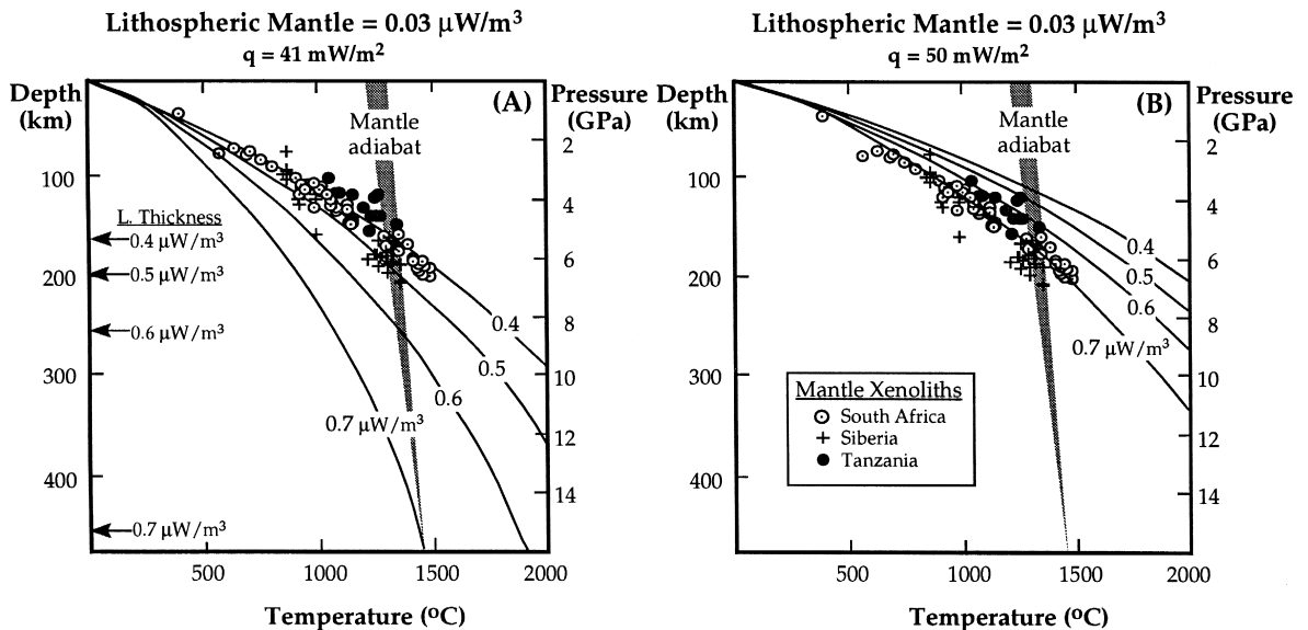
Fig. 6. (A) Conductive geotherms corresponding to surface heat flow of 41 \text{ mW/m}^2 for a variety of bulk crust compositions ( 0.4 to 0.7 \text{ }\mu\text{W/m}^3 ) and lithospheric mantle composition equal to our best estimate of cratonic peridotite ( 0.03 \text{ }\mu\text{W/m}^3 , column 10 of Table 5). Xenolith P – T points were calculated using the Brey and Köhler (1990) calibrations of the 2 pyroxene thermometer and Al in orthopyroxene barometer. Lithospheric thickness of the different models are marked on the left axis. Cratonic peridotite xenolith P – T data points fall between geotherms corresponding to crustal heat production of 0.4 to 0.5 \text{ }\mu\text{W/m}^3 , which corresponds to a lithospheric thickness of less than 200 \text{ km} . The most radiogenic crust composition at 0.7 \text{ }\mu\text{W/m}^3 corresponds to 12 \text{ mW/m}^2 heat flow across the Moho (equivalent to estimates for Moho heat flux in several Archean regions (e.g., Pinet and Jaupart, 1987, Pinet et al., 1991)), but requires a 450 \text{ km} thick lithosphere, which would extend into the Earth's transition zone. (B) Same as (A) but for 50 \text{ mW/m}^2 surface heat flow.
