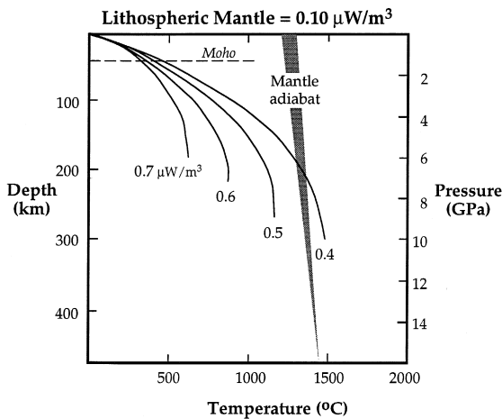
Fig. 5. Conductive geotherms corresponding to surface heat flow of 41 \text{ mW/m}^2 for a variety of bulk crust compositions ( 0.4 to 0.7 \text{ } \mu\text{W/m}^3 ) and lithospheric mantle composition equal to the average garnet peridotite from kimberlites ( 0.093 \text{ } \mu\text{W/m}^3 , or 0.15 \text{ wt\% K}_2\text{O} , Table 5 column 5). Only the geotherm for the least radiogenic crust composition ( 0.4 \text{ } \mu\text{W/m}^3 , corresponding to the heat production of average granulites) intersects the mantle adiabat.
