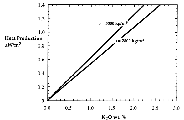
Fig. 1. K 2 O content (in weight %) versus heat production for two densities: 2800 kg/m 3 , representative of crustal rocks and 3300 kg/m 3 , representative of mantle peridotite, assuming K/U = 10,000 and Th/U = 3.9. Compositions that deviate from these assumed proportions of K, Th and U will not plot on these lines.
