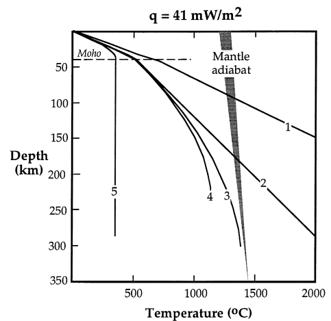
Fig. 3. Model geotherms illustrating the effects of various lithospheric heat source distributions for a surface heat flow of 41 mW/m 2 . Also shown is a range of mantle adiabats with which a reasonable geotherm should merge at the base of the lithosphere (see text). Curve 1 has no lithospheric heat sources, and intersects the adiabat at 85 km. Curve 5 produces all the surface heat flow from crustal heat sources; the temperature is constant with depth (and low) beneath the crust, and results in an unreasonable geotherm. For curves 2, 3, 4 half of the surface heat flow is produced in the crust. Curves 2 and 3 produce reasonable geotherms that meet the adiabat, but curve 4 has mantle heat sources that are too high, and it never reaches the adiabat. Other parameters as in Table 3.
