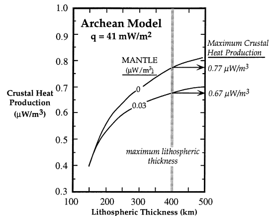
Fig. 7. Lithospheric depth (km) versus crustal heat production for Archean cratons where the surface heat flow is 41 \text{ mW}/\text{m}^2 . Two curves are illustrated: zero heat production in the lithospheric mantle and our preferred heat production of 0.03 \mu\text{W}/\text{m}^3 . Lithospheric thickness is defined by the intersection of conductive geotherms (calculated according to parameters in Table 4) with the mantle adiabat (see text). Arrows point to maximum crustal heat production for each model. These systematics demonstrate that the uppermost limit to heat production in Archean crust is 0.77 \mu\text{W}/\text{m}^3 , and lower values are probably more realistic (i.e., there is heat production in the lithospheric mantle and cratonic lithosphere is likely to be thinner than 400 km).
