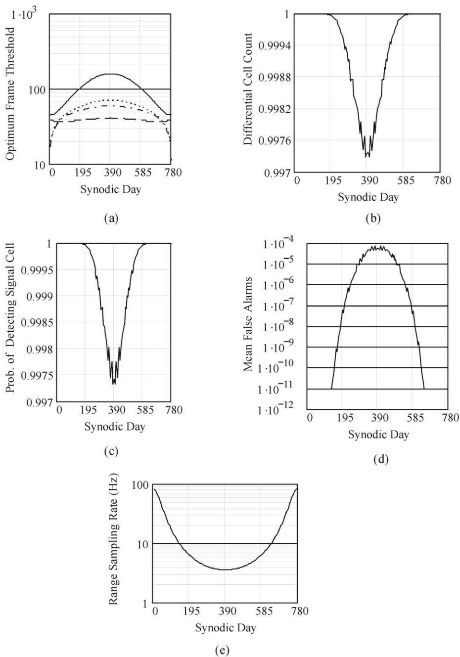
Fig. 11. Operating parameters as a function of synodic phase/day for the balanced, low SNR, photon-counting Earth–Mars transponder link operating at 2 kHz during initial acquisition under worst case conditions of unsynchronized clocks: (a) optimum detection threshold; (b) optimized differential cell count; (c) optimized signal detection probability; (d) mean false alarms per laser fire; and (e) range sampling rate. In (a), Earth daylight and night operations are indicated by the solid and dashed lines respectively whereas Mars daylight and night operations are represented by dotted and dash-dotted lines respectively. Because the link is “balanced”, the four curves in (b) through (d) overlap.
