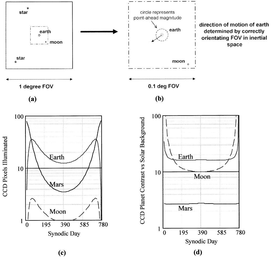
Fig. 8. (a) Simulated CCD camera display of a 1° by 1° FOV showing the centered Earth, Moon, and background stars used in the computation of the transmitter point ahead angle and direction. (b) The circle around the Earth represents the magnitude of the angular offset as computed from the planetary ephemerides, and the arrow represents the Earth's forward motion as determined by other celestial objects (Moon, stars) in the camera FOV. The intersection of these two curves indicates the desired laser beam pointing. Sampling of the outgoing laser beam by the prism assembly can provide pointing verification. (c) Number of CCD pixels illuminated at the viewing terminal by the Earth, Mars, and Moon as a function of synodic day; (d) Worst-case contrast of planetary image relative to background counts caused by solar scattering from the local atmosphere during daylight operations.
