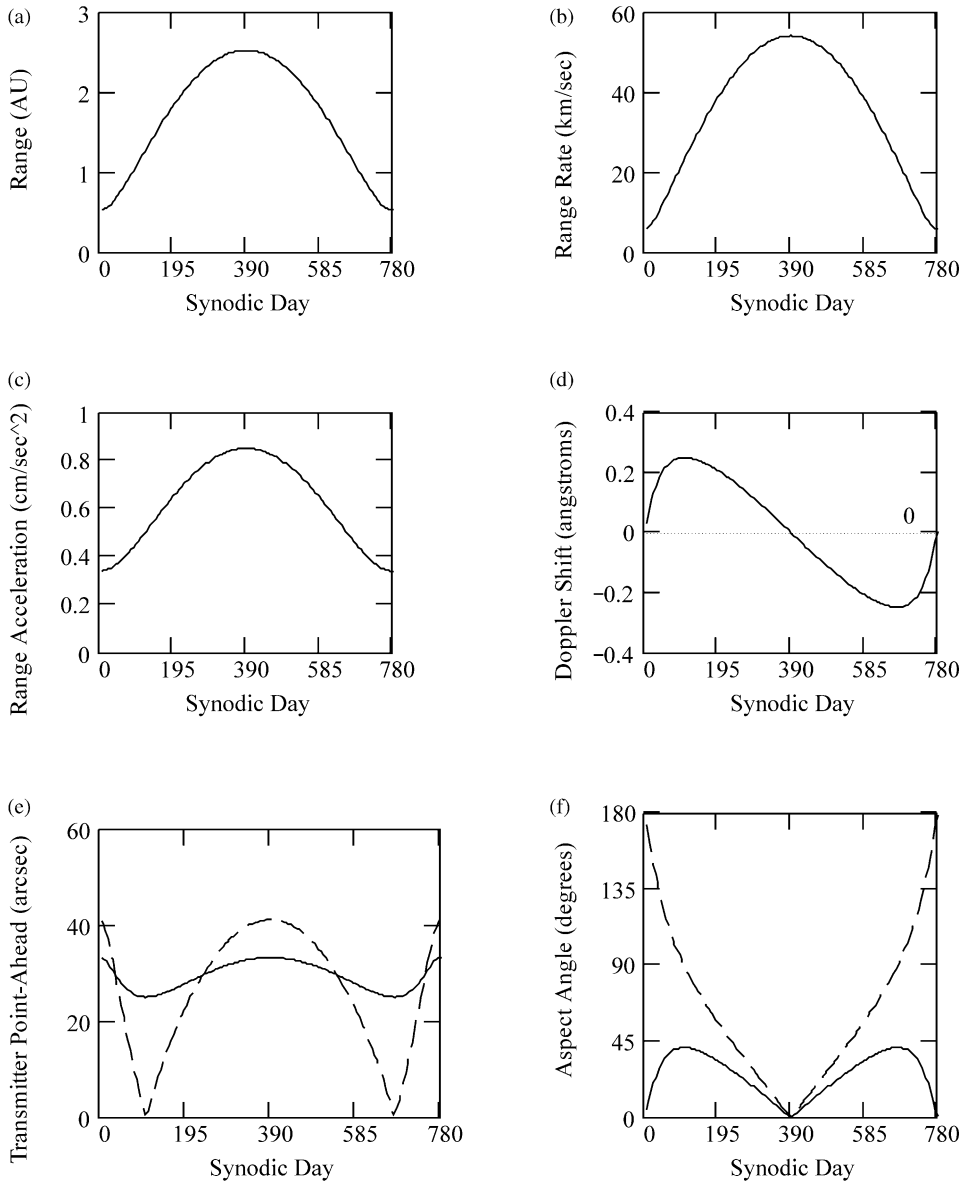
Fig. 9. Various plots relevant to the Earth–Mars link as a function of synodic phase/day: (a) range in AU; (b) range-rate in km/s; (c) range acceleration in cm/s 2 ; (d) Doppler shift in Angstroms; (e) transmitter point ahead angle in arc-seconds; and (f) aspect angles. In (e) and (f), the Earth terminal is represented by a solid line and the Mars terminal by a dashed line.
