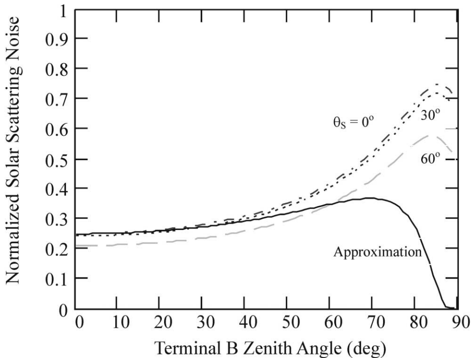
Fig. 4. Normalized contribution of local atmospheric scattering to the noise at Terminal A as a function of the Solar and Terminal B zenith angles, \theta_S ( 0^\circ , 30^\circ , 60^\circ ) and \theta_B ( 0 to 90^\circ ), respectively as computed using (14) in the text. A standard clear Earth atmosphere (visibility = 23 km) was assumed with a zenith transmission T_B = 0.7 . The solid line represents the approximation in (14) which is independent of the solar zenith angle and valid under the assumption of high atmospheric transmission ( T_B \sim 1 ) or \theta_S \sim \theta_B . The approximation is fairly good for \theta_B < 60^\circ and improves for clearer or more transmissive atmospheres.
