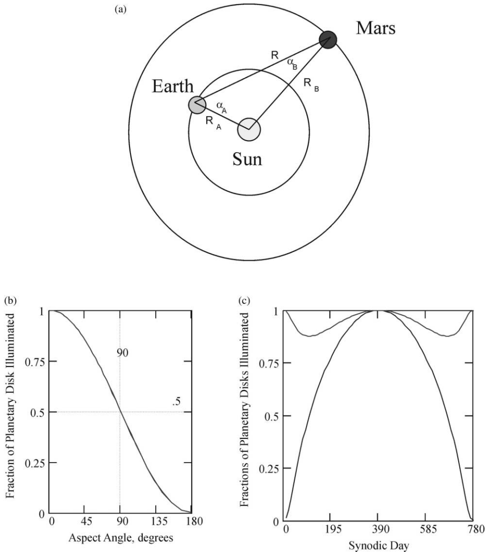
Fig. 3. (a) Solar system view of Planets A and B circling the Sun. The aspect angle for Planet A is defined as the angle formed by two vectors originating at Planet A and directed toward the other two bodies and vice versa. (b) The fraction of the planetary disk illuminated by the Sun as a function of aspect angle. (c) The fraction of the Earth (lower curve) and Mars (upper curve) disk illuminated by the Sun as viewed by the transponder terminals as a function of synodic phase (see Section 5). In our modeling of planetary albedo noise, each planet is assumed to be a solid sphere whose surface is characterized by a globally averaged surface reflectivity, \rho , with a thin atmospheric shell characterized by a zenith transmission, T . Planetary albedo noise is generated from any point on the planet where the solar illumination and receiver FOV overlap.
