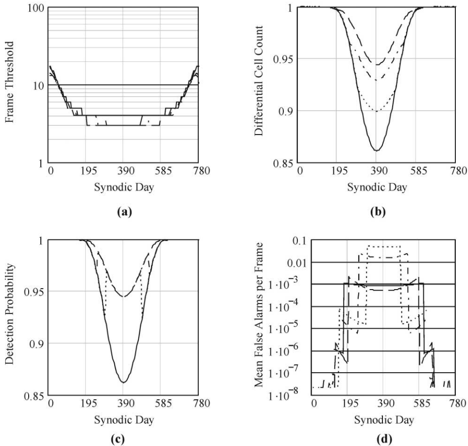
Fig. 10. Operating parameters as a function of synodic phase/day for the balanced, high SNR Earth–Mars transponder link operating at 5 Hz during initial acquisition under worst case conditions of unsynchronized clocks: (a) optimum detection threshold; (b) optimized differential cell count; (c) optimized signal detection probability; and (d) mean false alarms per laser fire. Earth daylight and night operations are indicated by the solid and dashed lines respectively; Mars daylight and night operations are represented by dotted and dash-dotted lines respectively.
