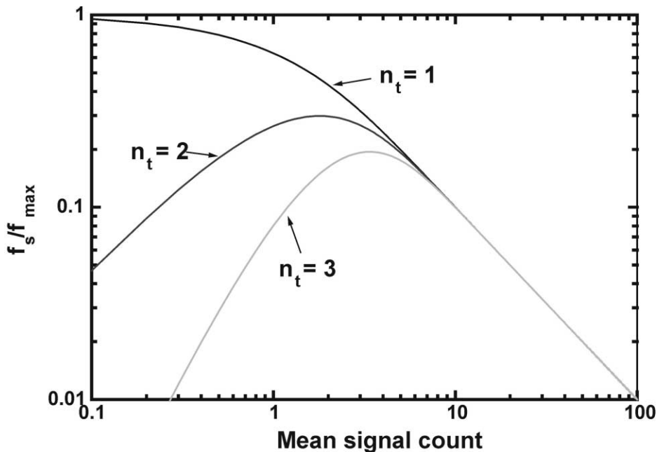
Fig. 2. Range sampling rate as a function of the detection threshold, n_t , and the mean signal count, n_s , normalized for a particular Mixed Power-Aperture Product and range.
