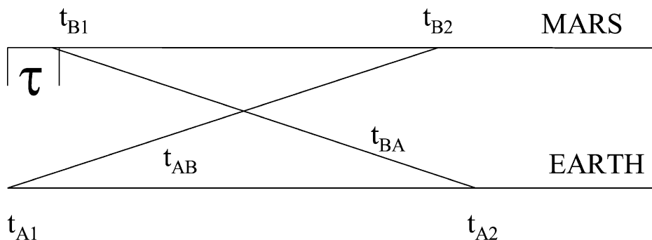
Fig. 1. Timing diagram for an asynchronous laser transponder on Mars exchanging pulses with an Earth station. A pulse leaves the Earth station at time t_{A1} , travels to Mars in a time t_{AB} , and arrives at Mars at time t_{B2} . Similarly, a pulse is transmitted from Mars at time t_{B1} , travels to Earth in a time t_{BA} , and arrives on Earth at time t_{A2} . Times of departure and arrival are referenced to that terminal's clock, and the Mars values are transmitted to Earth over a microwave or laser communications link. The quantity \tau is the actual time interval between the departure of pulses from the Earth and Mars stations and, combined with the outgoing pulse times as recorded by their respective clocks, provides the offset between the ground and spacecraft clocks.
