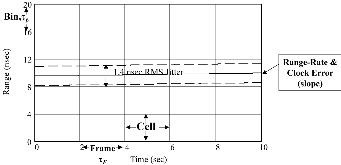
Fig. 5. The arrival times of incoming photons are recorded relative to when they are expected in an Observed Minus Calculated (O–C) plot. In this reference system, a Correlation Range Receiver (CRR) divides the range gate in the vertical axis into range bins and the sequence of laser fires along the horizontal axis into frames . The bin and frame sizes are chosen to ensure high probability that the observed signal counts all fall within a single cell , i.e. the 2-D areas defined by the vertical borders of the frame and the horizontal borders of the bins. The choice of bin and frame size are intertwined and must take into account the basic precision of the measurement, which sets a minimum bin size, as well as the time it takes to collect enough signal counts to adequately discriminate the signal cell from the noise cells . Various residual uncertainties in the range rate, due to ephemerides and planetary rotation model errors, as well as clock frequency offsets, which can mimic a range-rate error via the Doppler equation, can cause the signal photons to fall along a sloped line with the random scatter, caused by laser fire or receiver timing jitter, superimposed.
