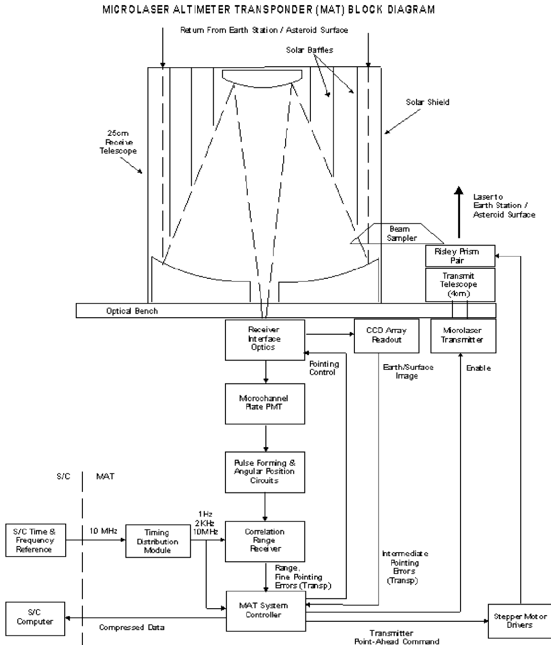
Fig. 7. Block diagram of a dual-mode Microlaser Altimeter Transponder (MAT) instrument. The CCD array is used to crudely center the planetary image within the quadrant photomultiplier FOV so that the latter can provide subarcsecond pointing corrections to maximize the link. A Risley prism pair is used to offset the transmitter line of sight for “point-ahead”. The accuracy of the point-ahead can be monitored by leaking a small portion of the outgoing pulse into the receiver and onto the CCD. The transponder can be used at any point during the mission, i.e. interplanetary cruise, in orbit, or the surface of another planet. While still in orbit, the same system can produce accurate 3-D topographic maps of the surface prior to landing and record coaligned 2-D visual images using the high resolution CCD camera.
