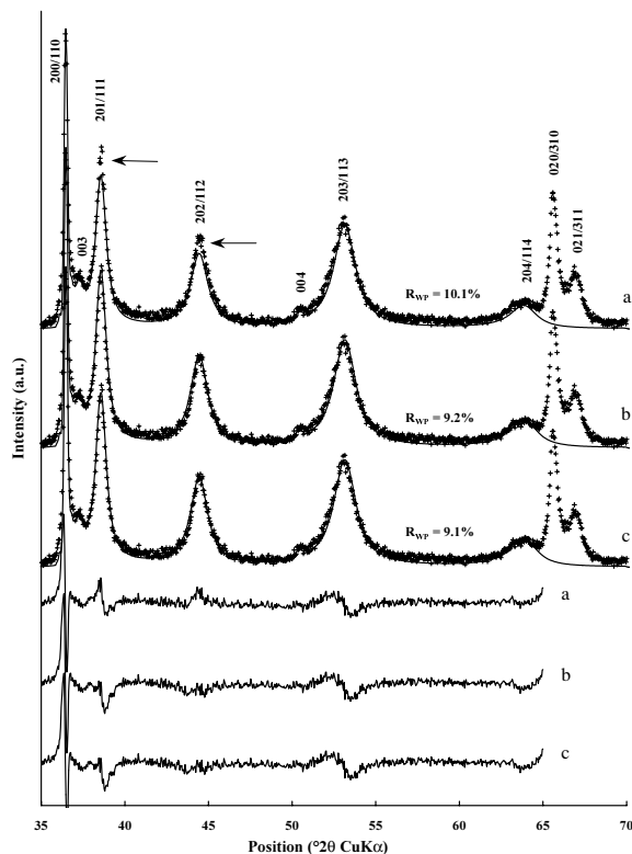
FIGURE 7. Comparison between experimental and calculated XRD patterns for PbBi 58 (top) and difference plots (bottom). Patterns as for Figure 2. Only 20/ and 11/ reflections are calculated. Atomic coordinates and other structural parameters used for the calculations are listed in Tables 2, 4, 5, and 6b. (a) Initial model in which all Mn interlayer (0.112 per octahedron) and Pb (0.054 per octahedron) are located only above or below vacant layer sites ( V TC sites). (b) Optimum model, with 0.044 and 0.010 Pb located in V TC and V TE sites, respectively. (c) Model in which the amount of Mn interlayer is increased to 0.123, as compared with the optimum 0.112 value. Distribution of Pb is similar to that of the optimal model.
