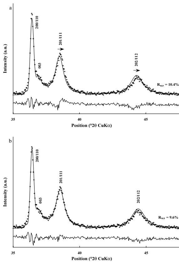
FIGURE 4. Comparison between experimental and calculated XRD patterns for CdBi 106 (top) and difference plots (bottom). Patterns as for Figure 2. Only 20l and 11l reflections are calculated. Atomic coordinates and other structural parameters used for the calculations are listed in Tables 2, 4, 5, and 6. (a) Defect-free (no well-defined stacking faults) 1H CdBi model. Positions of calculated 20l,11l_H and 202,112_H reflections are slightly shifted toward lower 2\theta values with respect to the corresponding experimental reflections (arrows). (b) Defective 1H CdBi model containing 7% of monoclinic layer pairs ( +a/3 shift between adjacent layers, Table 4).
