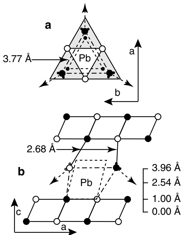
FIGURE 8. Schematic view of Pb site above/below empty tridentate cavities ( V TE site). ( x , y ) coordinates of this position are (−0.333, 0) above the lower layer and (0.333, 0) below this layer. All patterns as for Fig. 6. (a) Projection on the a - b plane. Small solid circles represent Mn layer from the lower layer. (b) Projection along the b axis.
