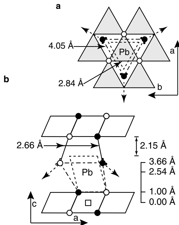
FIGURE 6. Schematic view of Pb site above/below vacant layer octahedra ( ^{\text{VI}}\text{TC} site). (x, y) coordinates of this position are (0, 0). (a) Projection on the a-b plane. The upper surface of the lower layer is shown as light shaded triangles. \text{O}_{\text{layer}} of this lower layer is shown as open circles. Dashed line outlines the ideal octahedron defined by the close packing of anions whereas irregular dashed line outlines the actual upper surface of the Pb octahedron, after further adjustment (arrows) of \text{H}_2\text{O} positions to obtain realistic Pb- \text{H}_2\text{O}_{\text{interlayer}} and \text{H}_2\text{O}_{\text{interlayer}}\text{-O}_{\text{layer}} distances. (b) Projection along the b axis. \text{O}_{\text{layer}} is shown as large circles. Open symbols indicate atoms at y = 0 , and solid symbols indicate atoms at y = \pm 1/2 . Vacant layer sites are shown as open squares and \text{Mn}_{\text{layer}} is not shown. Other patterns as Figure 6a. Z-coordinates of \text{Mn}_{\text{layer}} , \text{O}_{\text{layer}} , Pb, and \text{H}_2\text{O}_{\text{interlayer}} are indicated.
