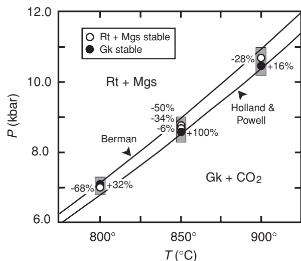
FIGURE 2. All experimental data from this study for reaction 3: \text{Rt} + \text{Mgs} = \text{Gk} + \text{CO}_2 . Filled circles, conditions at which Gk is stable; open circles, Rt + Mgs stable. The P plotted for each experiment has been corrected to the value for equilibrium between minerals and a pure CO 2 fluid (see Fig. 1 and text). Numbers refer to % reaction (positive values denote decarbonation; negative values carbonation). Size of circles represents the precision of the control of P and T during the experiments ( \pm 100 bars, \pm 2 °C). Shaded rectangles represent the preferred experimental estimate of the location of the equilibrium considering the size of the narrowest bracket at each T and uncertainties in the accuracy in P ( \pm 300 bars) and T ( \pm 3 °C). Solid curves are the P - T conditions for the equilibrium computed from the thermodynamic databases of Berman (1988, updated 1992) and Holland and Powell (1998, updated 2001).
