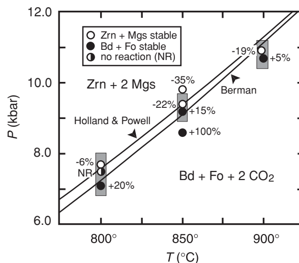
FIGURE 3. All experimental data from this study for reaction 4: \text{Zrn} + 2 \text{Mgs} = \text{Bd} + \text{Fo} + 2 \text{CO}_2 . Filled circles, conditions at which Bd + Fo is stable; open circles, Zrn + Mgs stable; half-filled circle, no reaction. All other features the same as in Figure 2.
