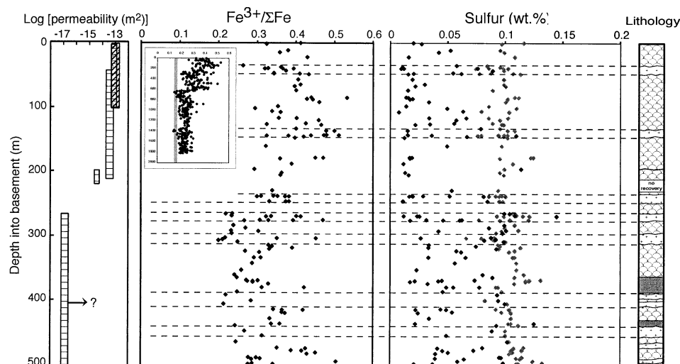
Fig. 2. Downhole profiles of \text{Fe}^{3+}/\Sigma\text{Fe} and S in Hole 504B down to 500 m subbasement. The inset shows the complete profile for Hole 504B with a preoxidative \text{Fe}^{3+}/\Sigma\text{Fe} of 0.15 marked by a vertical gray line. Gray symbols are prealteration sulfur contents calculated (see text). Dashed lines mark positions of massive lava flows that are typically less oxidized. Permeability data are from Fisher (1998).
