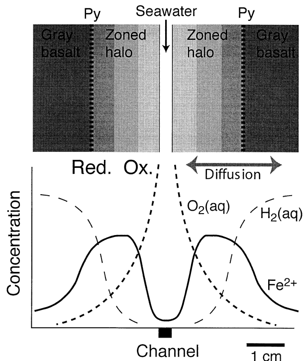
Fig. 7. Simplified view of an alteration halo parallel to a fluid conduit in the upper ocean crust. Oxidizing agents diffuse into the rock, while the pore fluids away from the conduit may become enriched in \text{Fe}(\text{II}) and \text{H}_2 as olivine/glass dissolution and hydrolysis proceed. Fe in the pore water diffuses down the concentration gradient into oxyhydroxide-rich, red bands (Fe-oxidation), leading to a pronounced redistribution of Fe within the alteration halo. As \text{H}_2 in the pore water increases away from the fracture, \text{Fe}(\text{III}) or sulfate may be reduced, possibly leading to the development of black, pyrite-rich bands in the rock.
