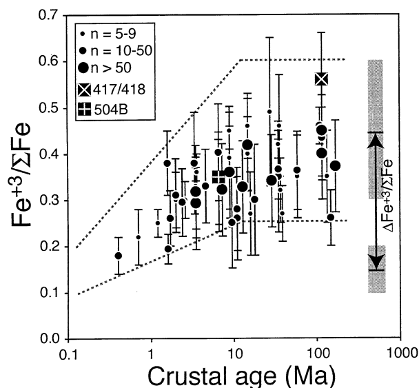
Fig. 3. Plot of average \text{Fe}^{3+}/\Sigma\text{Fe} of altered basalt samples versus basement age. Data are from Johnson and Semyan (1994) and Table 3. Each circles represents the unweighted average for an entire bore hole with 2\sigma standard deviation indicated by the error bars. Weighted averages are represented by solid squares. The symbol size varies with the number of analyses available for individual holes (see inset). There is a weak correlation between \text{Fe}^{3+}/\Sigma\text{Fe} and crustal age suggesting that \text{Fe}^{3+}/\Sigma\text{Fe} predominantly increases within the first 10 to 20 Myr of crustal evolution.
