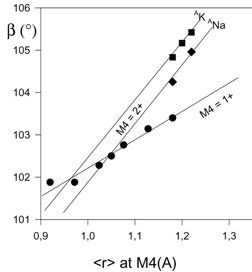
FIGURE 3. Relation between \beta and the mean ionic radius at M4 for some synthetic amphiboles. Circles = this work; squares = 8 K substituted potassium-richterite; diamonds = 8 Sr substituted sodium-richterite; data from Robert et al. (1993).
