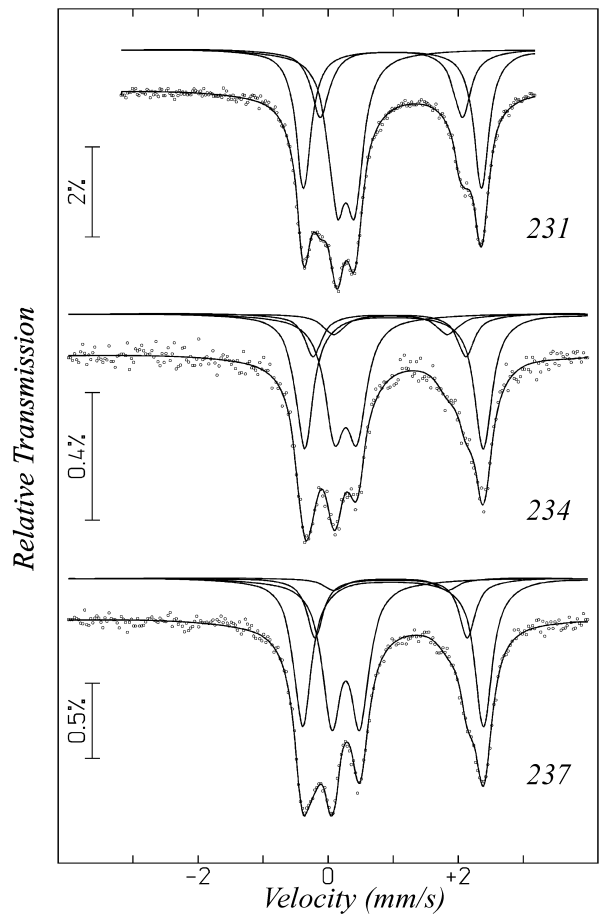
FIGURE 4. Mössbauer spectra of the two end-members and the 50:50 composition along the ferri-clinoferroholmquistite-riebeckite join.
