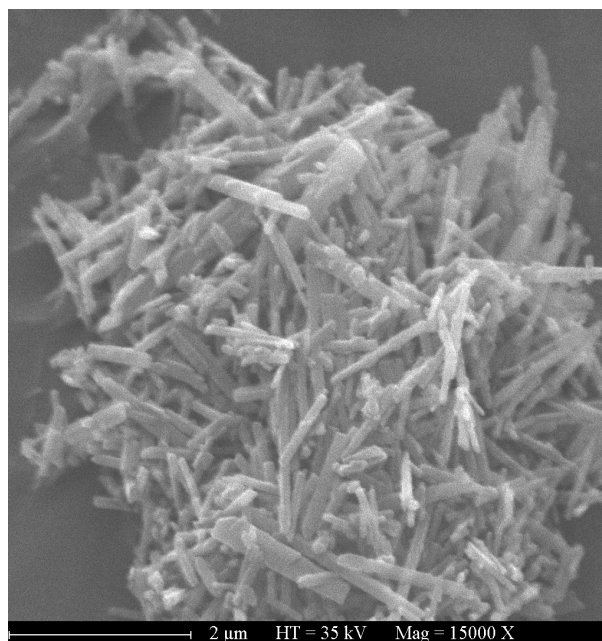
FIGURE 1. SEM image of synthetic end-member riebeckite (sample 237). The scale bar is 2 \mu\text{m} . The amphibole crystals are acicular and between 0.1–0.2 \mu\text{m} across and 0.5 to 2 \mu\text{m} long.
