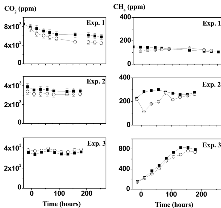
Figure 4. Total \text{CO}_2 and \text{CH}_4 emission of the enriched plant (■) and reference plant (○) during experiment 1, 2 and 3. The \text{CO}_2 concentrations were determined at the end of the night period. During day time the \text{CO}_2 concentration dropped to zero due to photosynthesis. ^{13}\text{CH}_4 is injected at t = 0 .
